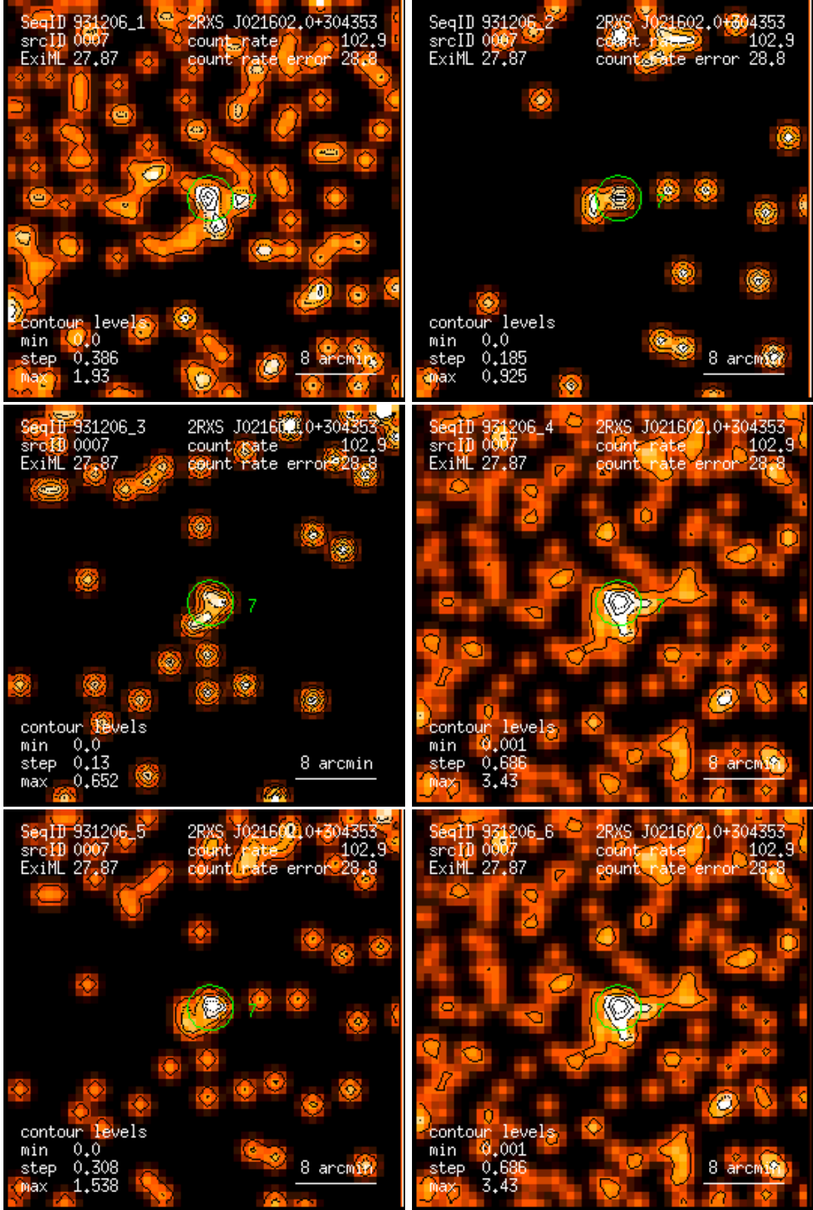
Figure 7: RASS 931206: detection 0007: band rate images, Gaussian filter: (1) PSPC channels 11 – 41, (2) 52 – 90, (3) 91 – 201, (4) 11 – 235, (5) 52 – 201, (6) 11 – 201. Broad band rates in counts/ks. Band rate contour levels in counts/ks/arcmin 2 .
