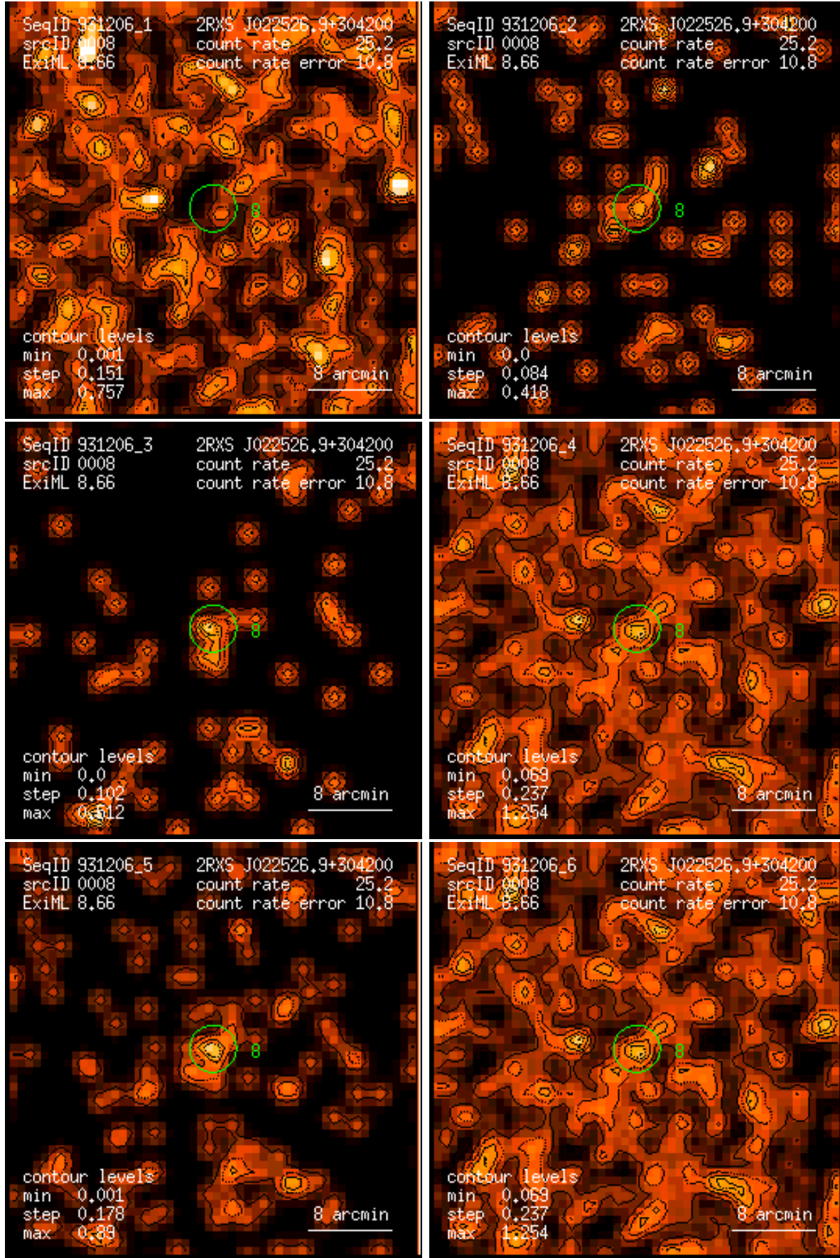
Figure 8: RASS 931206: detection 0008: band rate images, Gaussian filter: (1) PSPC channels 11 – 41, (2) 52 – 90, (3) 91 – 201, (4) 11 – 235, (5) 52 – 201, (6) 11 – 201. Broad band rates in counts/ks. Band rate contour levels in counts/ks/arcmin 2 .
