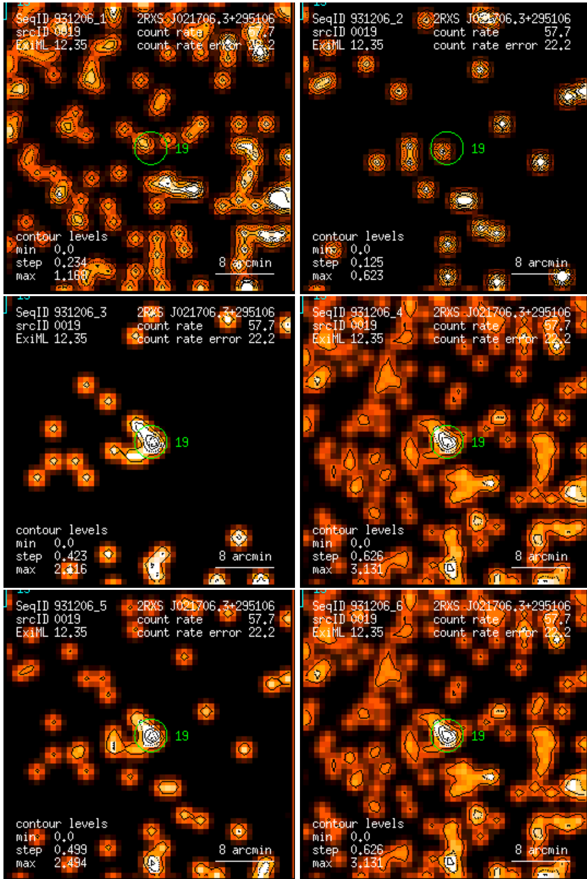
Figure 19: RASS 931206: detection 0019: band rate images, Gaussian filter: (1) PSPC channels 11 – 41, (2) 52 – 90, (3) 91 – 201, (4) 11 – 235, (5) 52 – 201, (6) 11 – 201. Broad band rates in counts/ks. Band rate contour levels in counts/ks/arcmin 2 .
