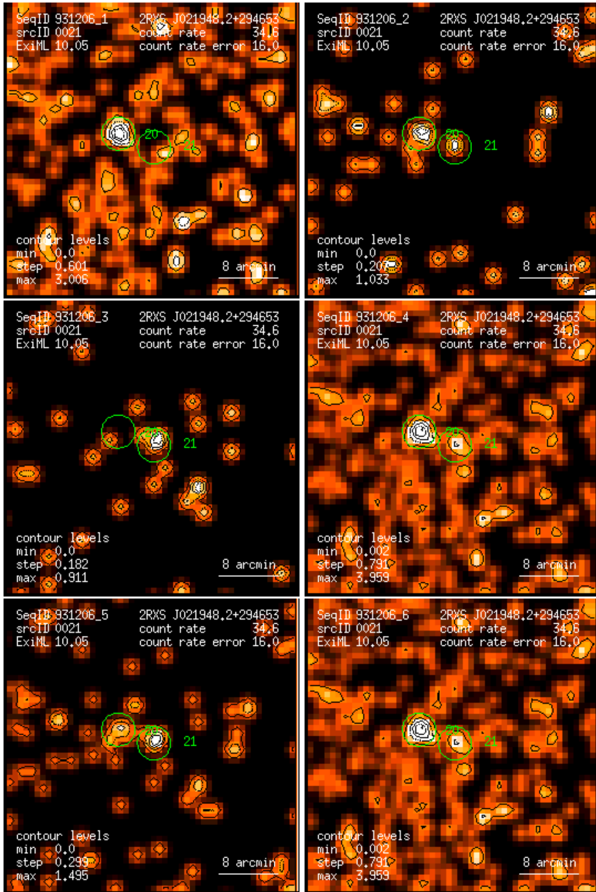
Figure 21: RASS 931206: detection 0021: band rate images, Gaussian filter: (1) PSPC channels 11 – 41, (2) 52 – 90, (3) 91 – 201, (4) 11 – 235, (5) 52 – 201, (6) 11 – 201. Broad band rates in counts/ks. Band rate contour levels in counts/ks/arcmin 2 .
