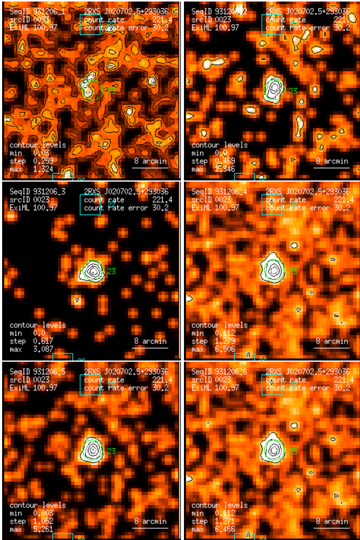
Figure 23: RASS 931206: detection 0023: band rate images, Gaussian filter: (1) PSPC channels 11 – 41, (2) 52 – 90, (3) 91 – 201, (4) 11 – 235, (5) 52 – 201, (6) 11 – 201. Broad band rates in counts/ks. Band rate contour levels in counts/ks/arcmin 2 .
