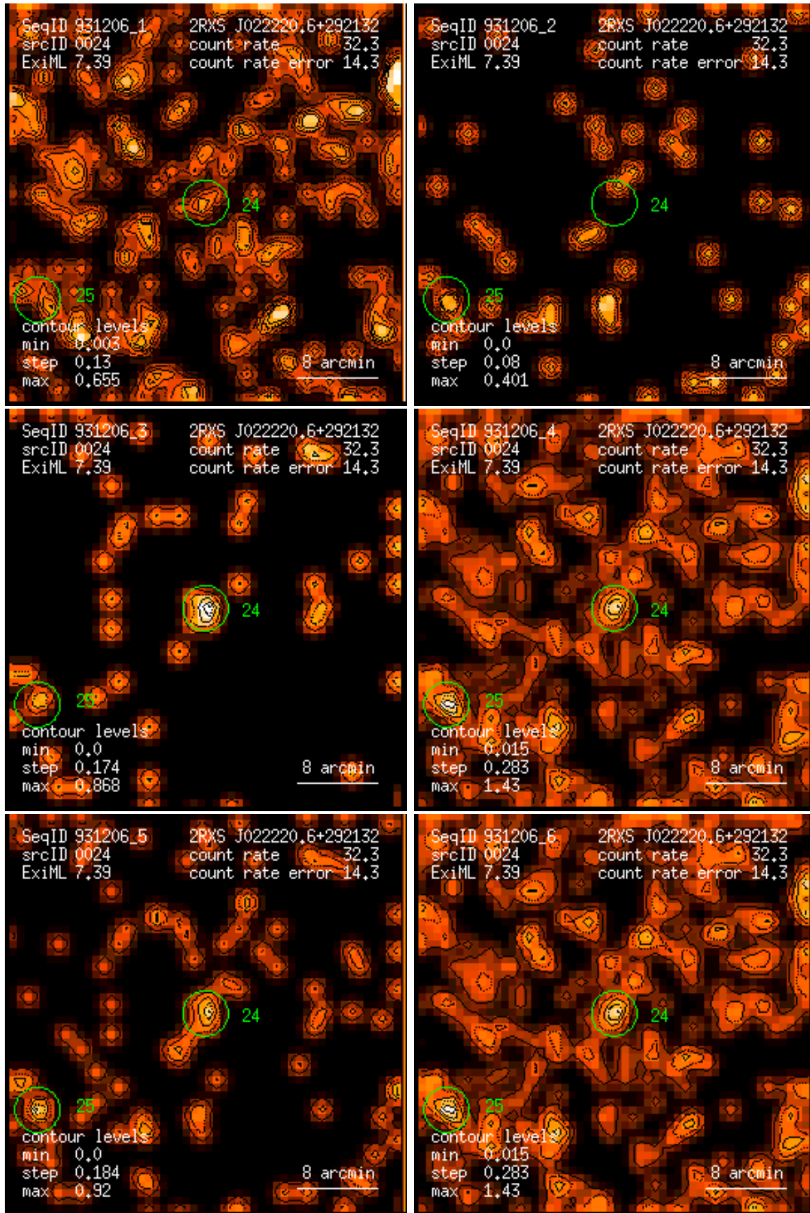
Figure 24: RASS 931206: detection 0024: band rate images, Gaussian filter: (1) PSPC channels 11 – 41, (2) 52 – 90, (3) 91 – 201, (4) 11 – 235, (5) 52 – 201, (6) 11 – 201. Broad band rates in counts/ks. Band rate contour levels in counts/ks/arcmin 2 .
