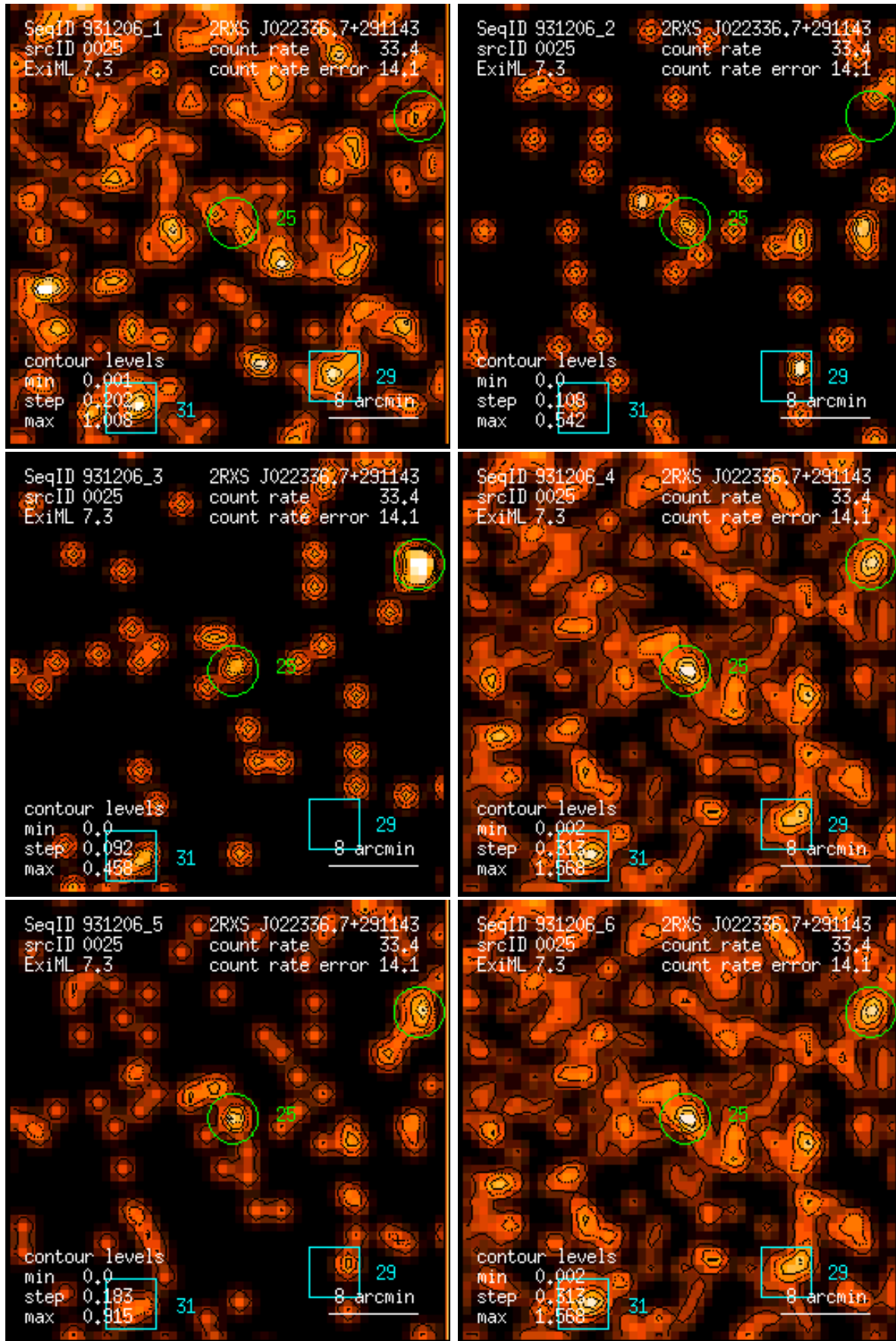
Figure 25: RASS 931206: detection 0025: band rate images, Gaussian filter: (1) PSPC channels 11 – 41, (2) 52 – 90, (3) 91 – 201, (4) 11 – 235, (5) 52 – 201, (6) 11 – 201. Broad band rates in counts/ks. Band rate contour levels in counts/ks/arcmin 2 .
