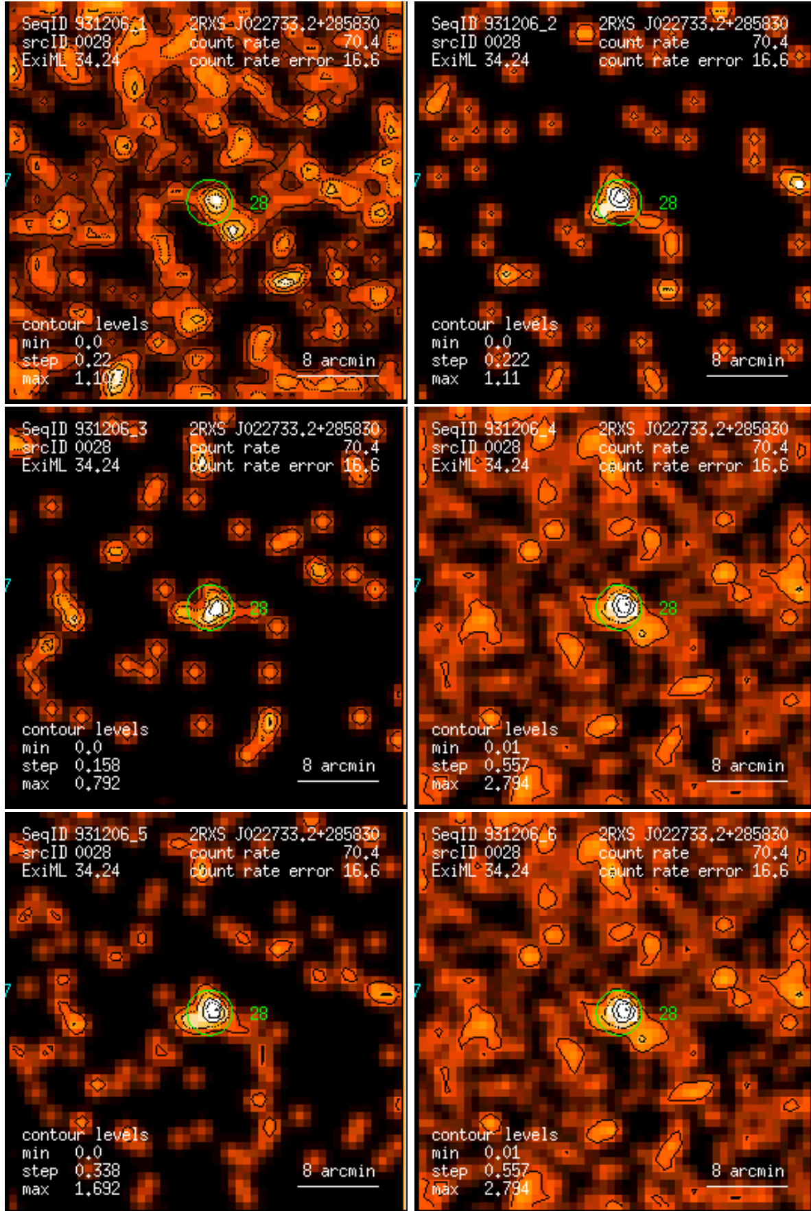
Figure 28: RASS 931206: detection 0028: band rate images, Gaussian filter: (1) PSPC channels 11 – 41, (2) 52 – 90, (3) 91 – 201, (4) 11 – 235, (5) 52 – 201, (6) 11 – 201. Broad band rates in counts/ks. Band rate contour levels in counts/ks/arcmin 2 .
