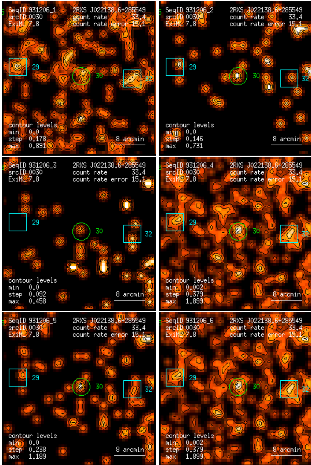
Figure 30: RASS 931206: detection 0030: band rate images, Gaussian filter: (1) PSPC channels 11 – 41, (2) 52 – 90, (3) 91 – 201, (4) 11 – 235, (5) 52 – 201, (6) 11 – 201. Broad band rates in counts/ks. Band rate contour levels in counts/ks/arcmin 2 .
