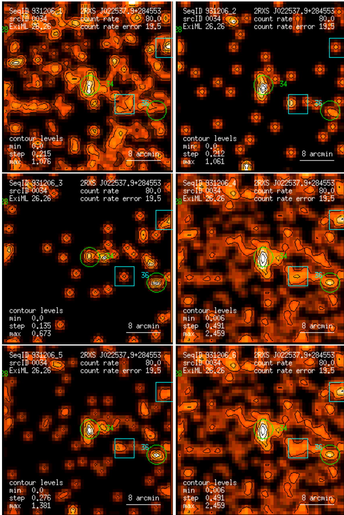
Figure 34: RASS 931206: detection 0034: band rate images, Gaussian filter: (1) PSPC channels 11 – 41, (2) 52 – 90, (3) 91 – 201, (4) 11 – 235, (5) 52 – 201, (6) 11 – 201. Broad band rates in counts/ks. Band rate contour levels in counts/ks/arcmin 2 .
