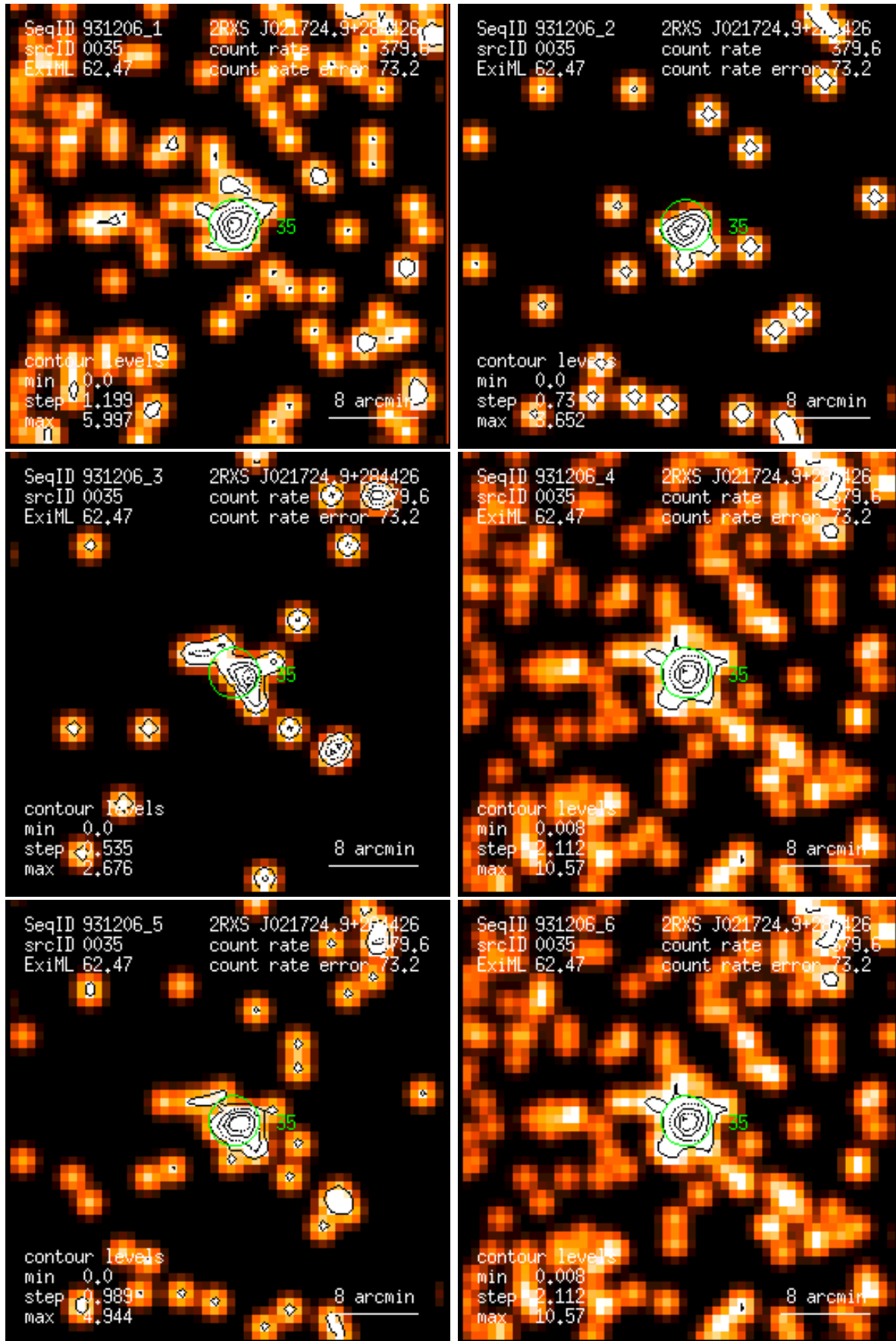
Figure 35: RASS 931206: detection 0035: band rate images, Gaussian filter: (1) PSPC channels 11 – 41, (2) 52 – 90, (3) 91 – 201, (4) 11 – 235, (5) 52 – 201, (6) 11 – 201. Broad band rates in counts/ks. Band rate contour levels in counts/ks/arcmin 2 .
