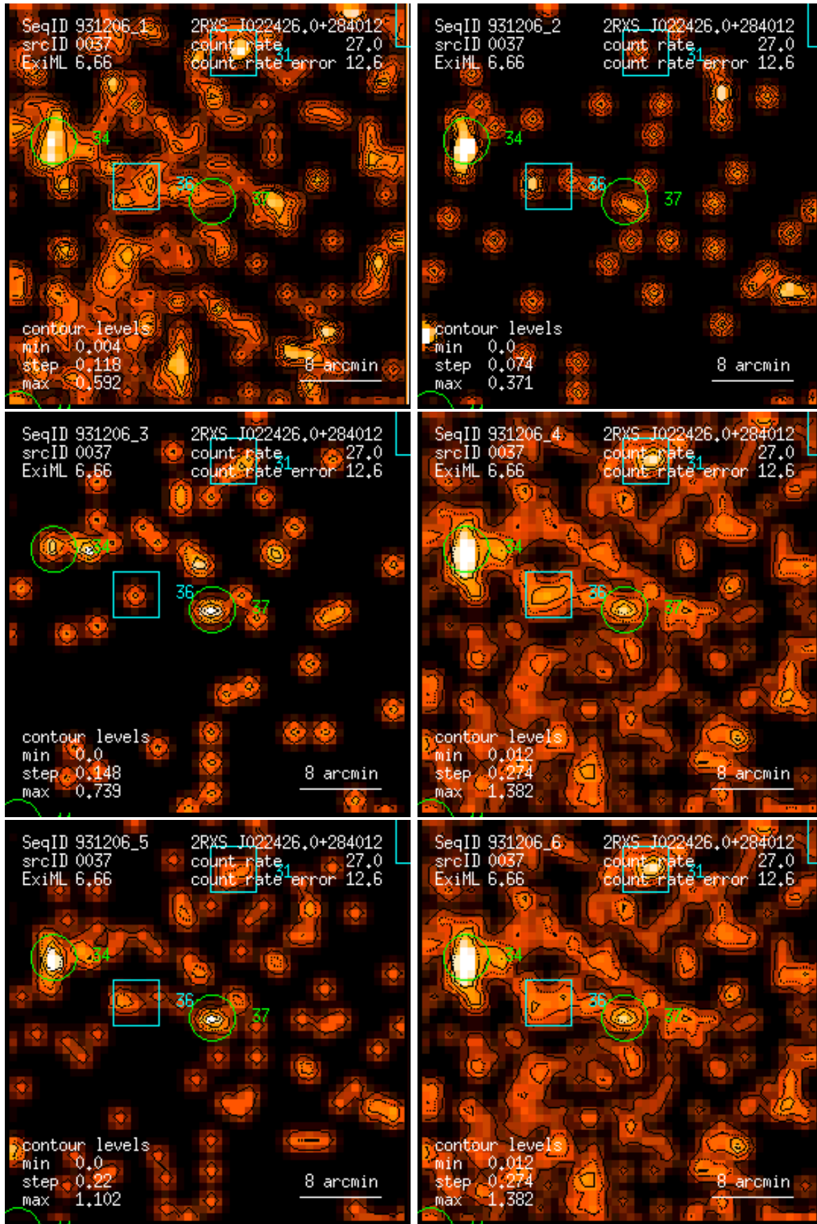
Figure 37: RASS 931206: detection 0037: band rate images, Gaussian filter: (1) PSPC channels 11 – 41, (2) 52 – 90, (3) 91 – 201, (4) 11 – 235, (5) 52 – 201, (6) 11 – 201. Broad band rates in counts/ks. Band rate contour levels in counts/ks/arcmin 2 .
