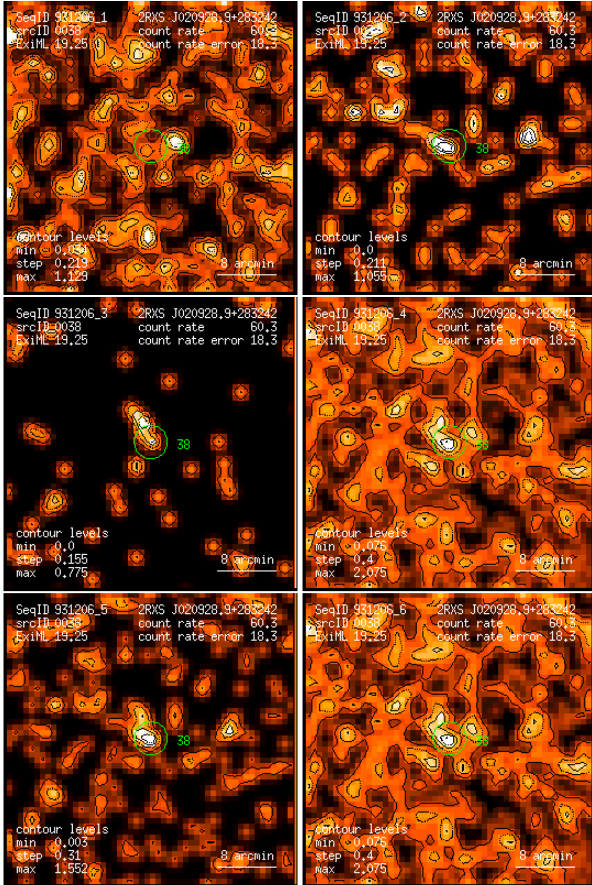
Figure 38: RASS 931206: detection 0038: band rate images, Gaussian filter: (1) PSPC channels 11 – 41, (2) 52 – 90, (3) 91 – 201, (4) 11 – 235, (5) 52 – 201, (6) 11 – 201. Broad band rates in counts/ks. Band rate contour levels in counts/ks/arcmin 2 .
