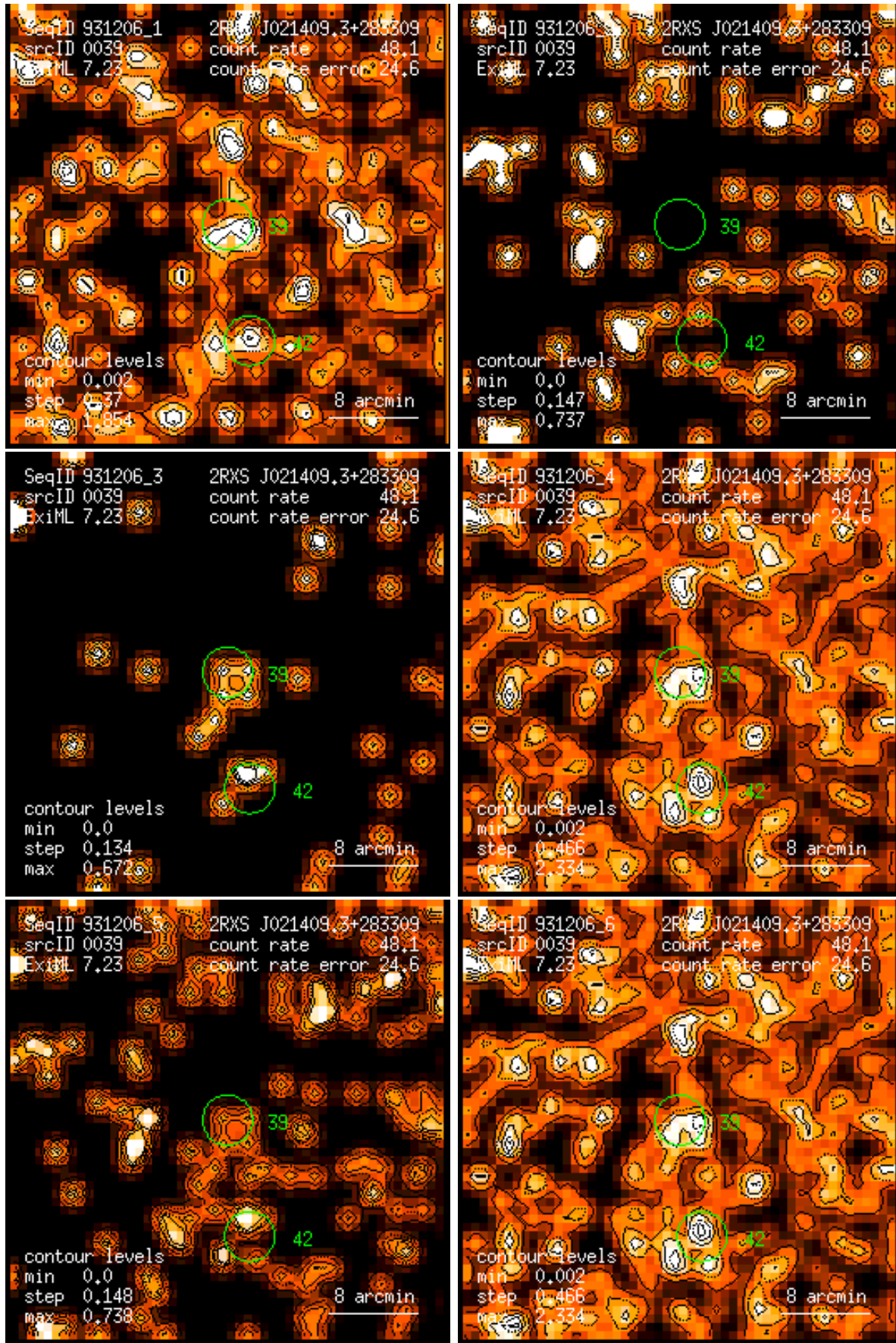
Figure 39: RASS 931206: detection 0039: band rate images, Gaussian filter: (1) PSPC channels 11 – 41, (2) 52 – 90, (3) 91 – 201, (4) 11 – 235, (5) 52 – 201, (6) 11 – 201. Broad band rates in counts/ks. Band rate contour levels in counts/ks/arcmin 2 .
