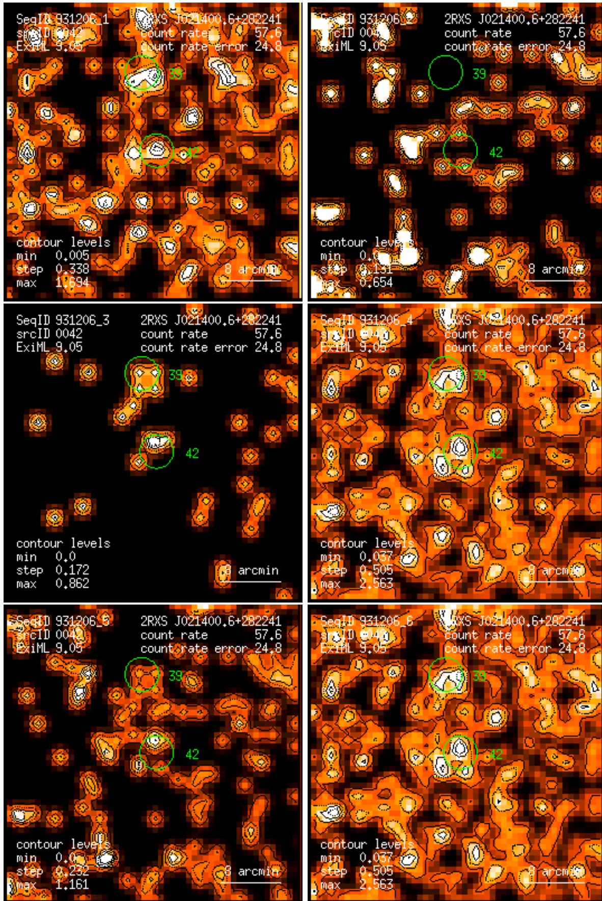
Figure 42: RASS 931206: detection 0042: band rate images, Gaussian filter: (1) PSPC channels 11 – 41, (2) 52 – 90, (3) 91 – 201, (4) 11 – 235, (5) 52 – 201, (6) 11 – 201. Broad band rates in counts/ks. Band rate contour levels in counts/ks/arcmin 2 .
