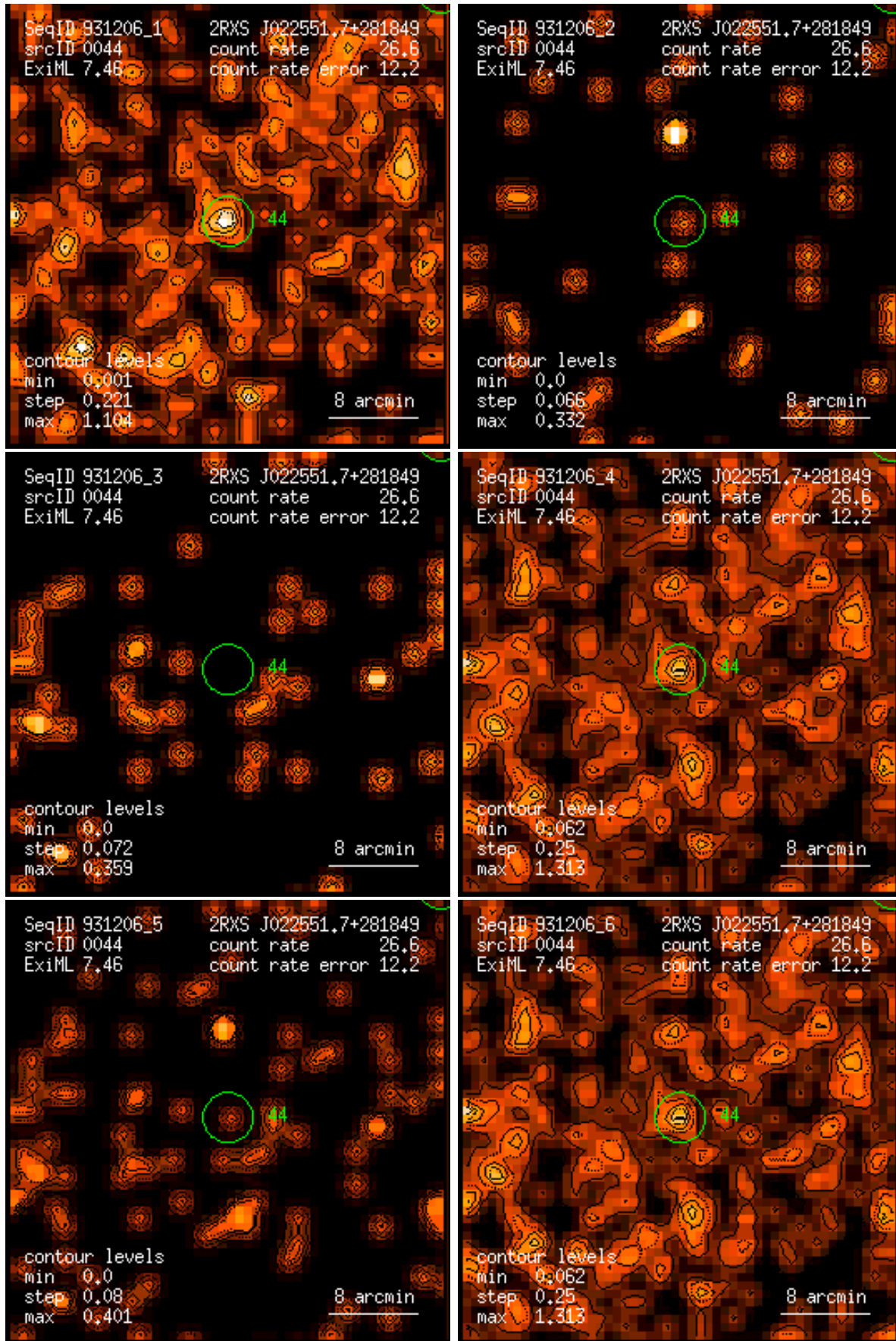
Figure 44: RASS 931206: detection 0044: band rate images, Gaussian filter: (1) PSPC channels 11 – 41, (2) 52 – 90, (3) 91 – 201, (4) 11 – 235, (5) 52 – 201, (6) 11 – 201. Broad band rates in counts/ks. Band rate contour levels in counts/ks/arcmin 2 .
