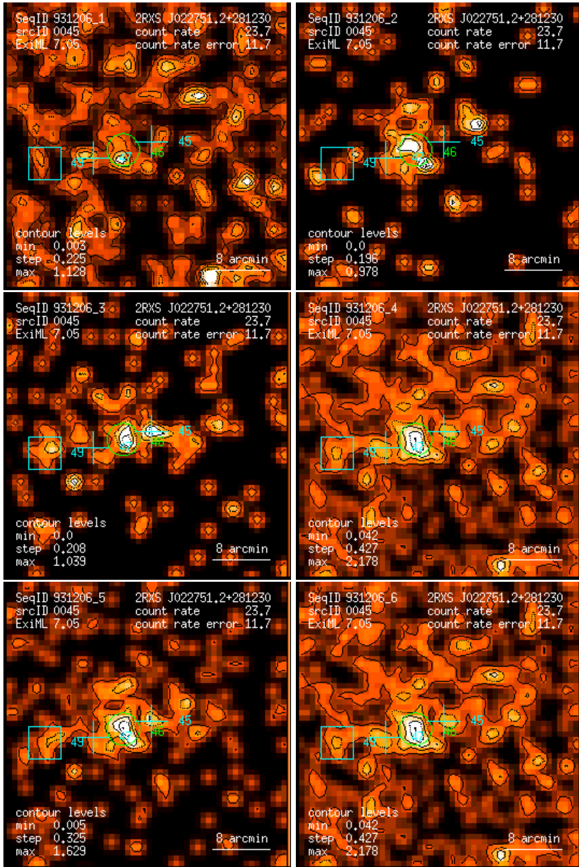
Figure 45: RASS 931206: detection 0045: band rate images, Gaussian filter: (1) PSPC channels 11 – 41, (2) 52 – 90, (3) 91 – 201, (4) 11 – 235, (5) 52 – 201, (6) 11 – 201. Broad band rates in counts/ks. Band rate contour levels in counts/ks/arcmin 2 .
