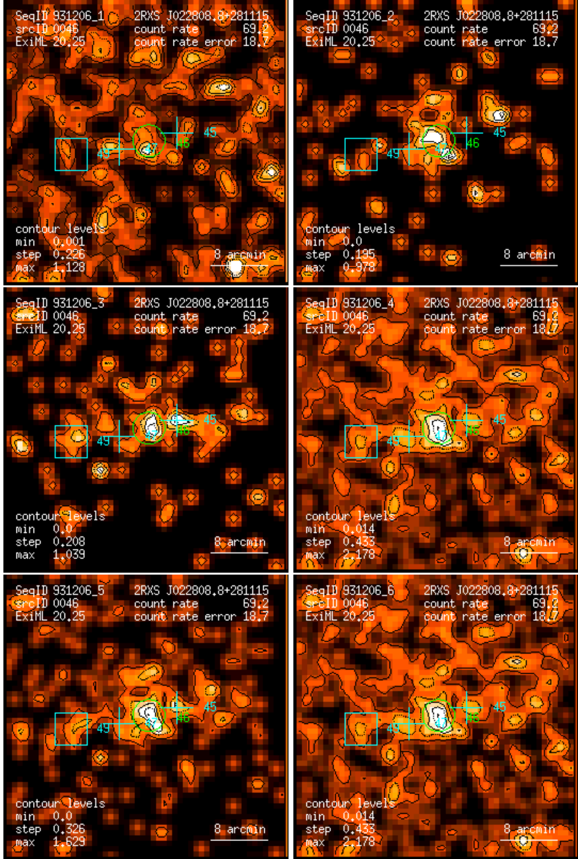
Figure 46: RASS 931206: detection 0046: band rate images, Gaussian filter: (1) PSPC channels 11 – 41, (2) 52 – 90, (3) 91 – 201, (4) 11 – 235, (5) 52 – 201, (6) 11 – 201. Broad band rates in counts/ks. Band rate contour levels in counts/ks/arcmin 2 .
