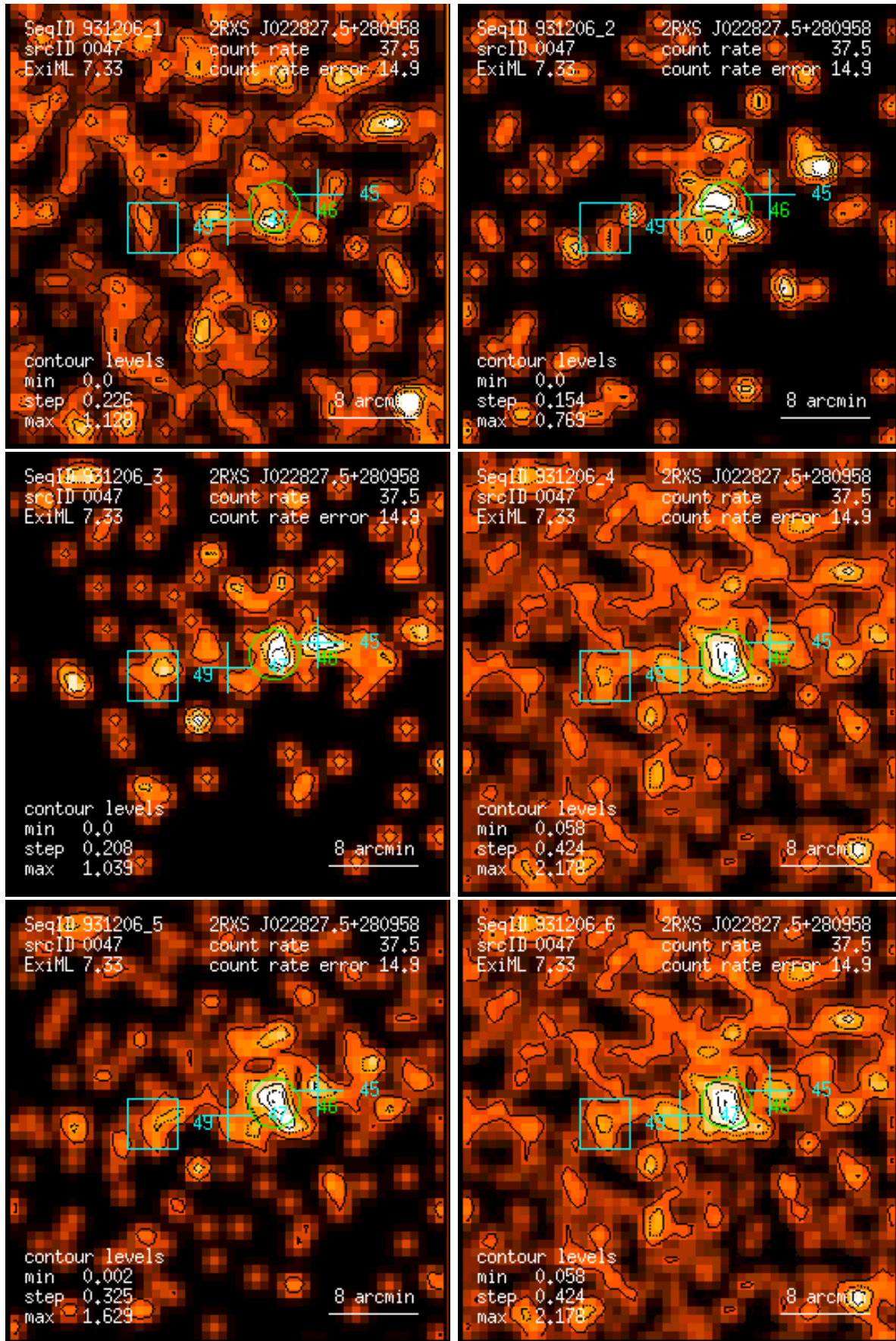
Figure 47: RASS 931206: detection 0047: band rate images, Gaussian filter: (1) PSPC channels 11 – 41, (2) 52 – 90, (3) 91 – 201, (4) 11 – 235, (5) 52 – 201, (6) 11 – 201. Broad band rates in counts/ks. Band rate contour levels in counts/ks/arcmin 2 .
