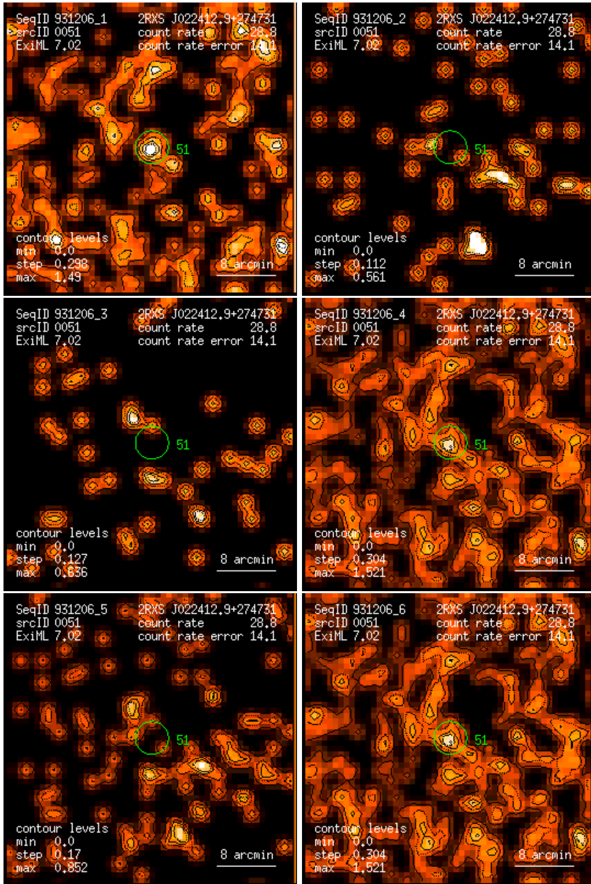
Figure 51: RASS 931206: detection 0051: band rate images, Gaussian filter: (1) PSPC channels 11 – 41, (2) 52 – 90, (3) 91 – 201, (4) 11 – 235, (5) 52 – 201, (6) 11 – 201. Broad band rates in counts/ks. Band rate contour levels in counts/ks/arcmin 2 .
