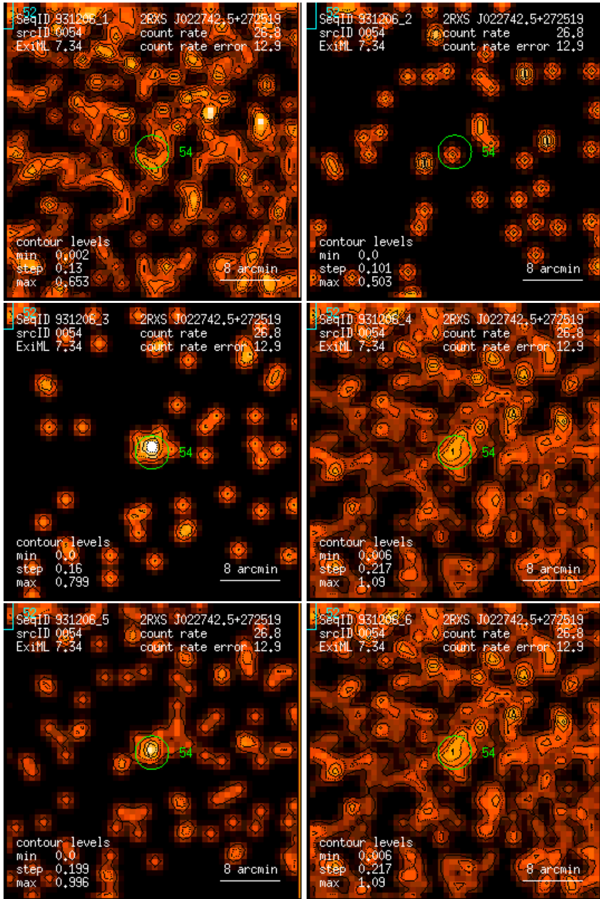
Figure 54: RASS 931206: detection 0054: band rate images, Gaussian filter: (1) PSPC channels 11 – 41, (2) 52 – 90, (3) 91 – 201, (4) 11 – 235, (5) 52 – 201, (6) 11 – 201. Broad band rates in counts/ks. Band rate contour levels in counts/ks/arcmin 2 .
