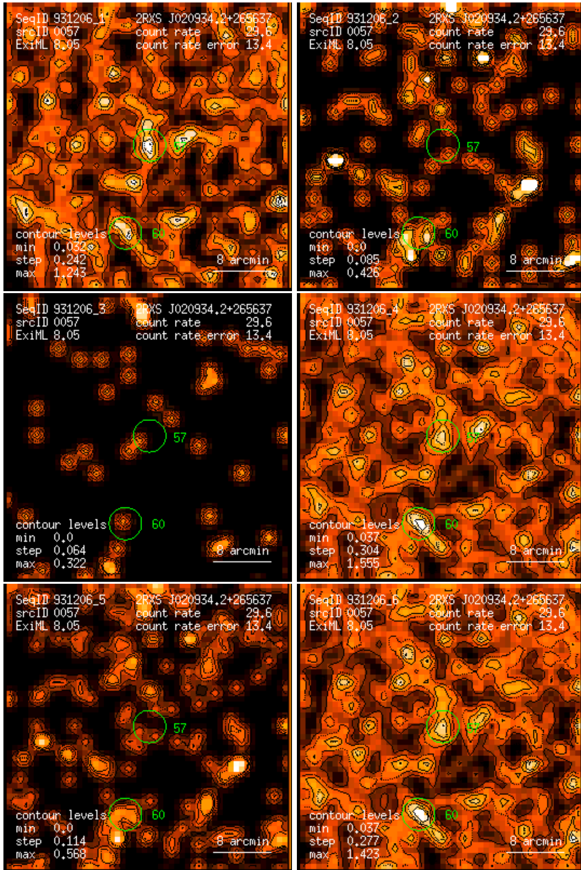
Figure 57: RASS 931206: detection 0057: band rate images, Gaussian filter: (1) PSPC channels 11 – 41, (2) 52 – 90, (3) 91 – 201, (4) 11 – 235, (5) 52 – 201, (6) 11 – 201. Broad band rates in counts/ks. Band rate contour levels in counts/ks/arcmin 2 .
