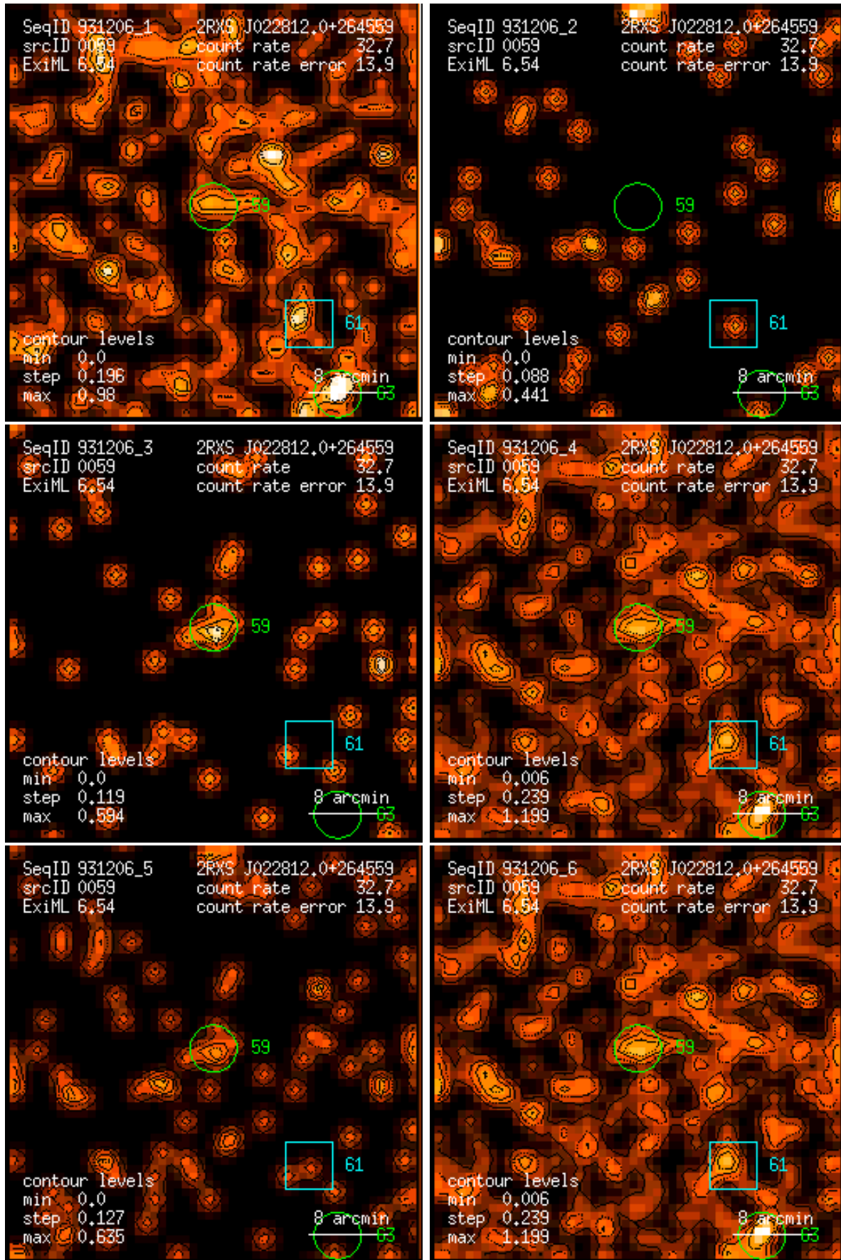
Figure 59: RASS 931206: detection 0059: band rate images, Gaussian filter: (1) PSPC channels 11 – 41, (2) 52 – 90, (3) 91 – 201, (4) 11 – 235, (5) 52 – 201, (6) 11 – 201. Broad band rates in counts/ks. Band rate contour levels in counts/ks/arcmin 2 .
