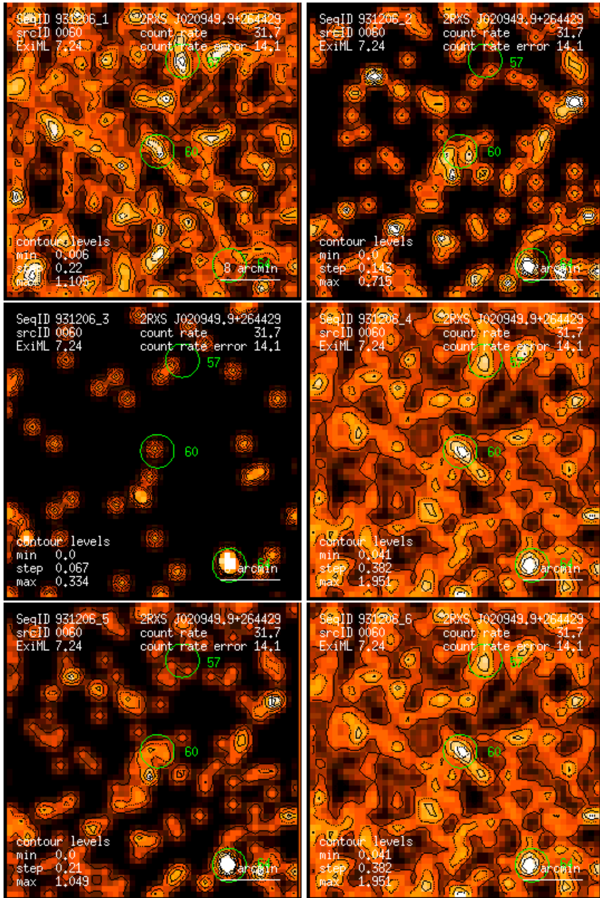
Figure 60: RASS 931206: detection 0060: band rate images, Gaussian filter: (1) PSPC channels 11 – 41, (2) 52 – 90, (3) 91 – 201, (4) 11 – 235, (5) 52 – 201, (6) 11 – 201. Broad band rates in counts/ks. Band rate contour levels in counts/ks/arcmin 2 .
