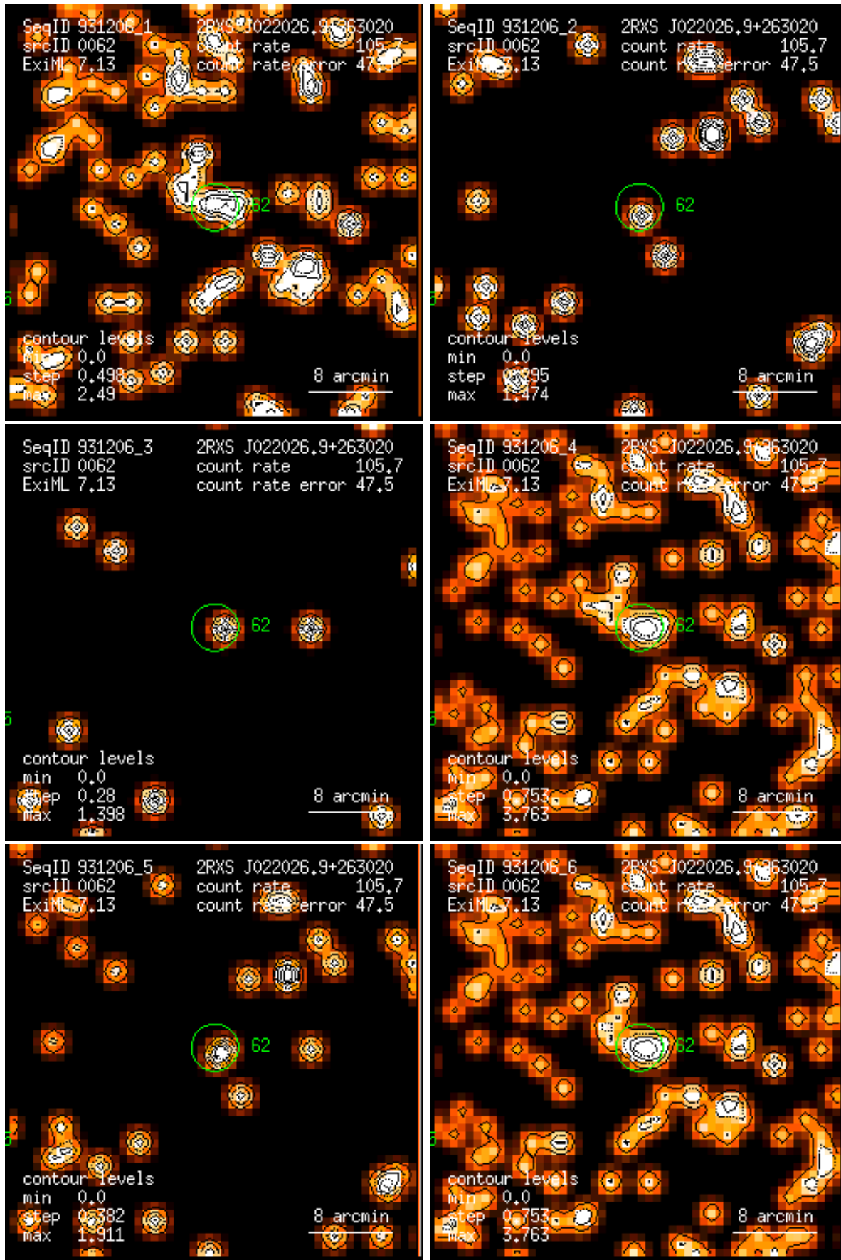
Figure 62: RASS 931206: detection 0062: band rate images, Gaussian filter: (1) PSPC channels 11 – 41, (2) 52 – 90, (3) 91 – 201, (4) 11 – 235, (5) 52 – 201, (6) 11 – 201. Broad band rates in counts/ks. Band rate contour levels in counts/ks/arcmin 2 .
