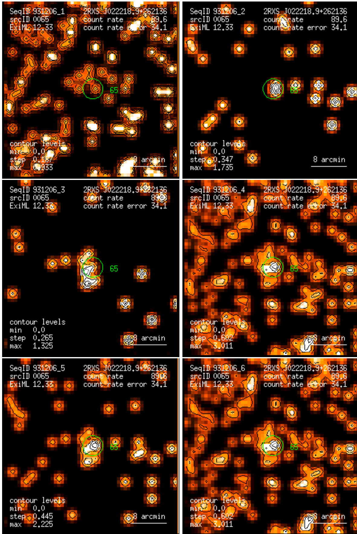
Figure 65: RASS 931206: detection 0065: band rate images, Gaussian filter: (1) PSPC channels 11 – 41, (2) 52 – 90, (3) 91 – 201, (4) 11 – 235, (5) 52 – 201, (6) 11 – 201. Broad band rates in counts/ks. Band rate contour levels in counts/ks/arcmin 2 .
