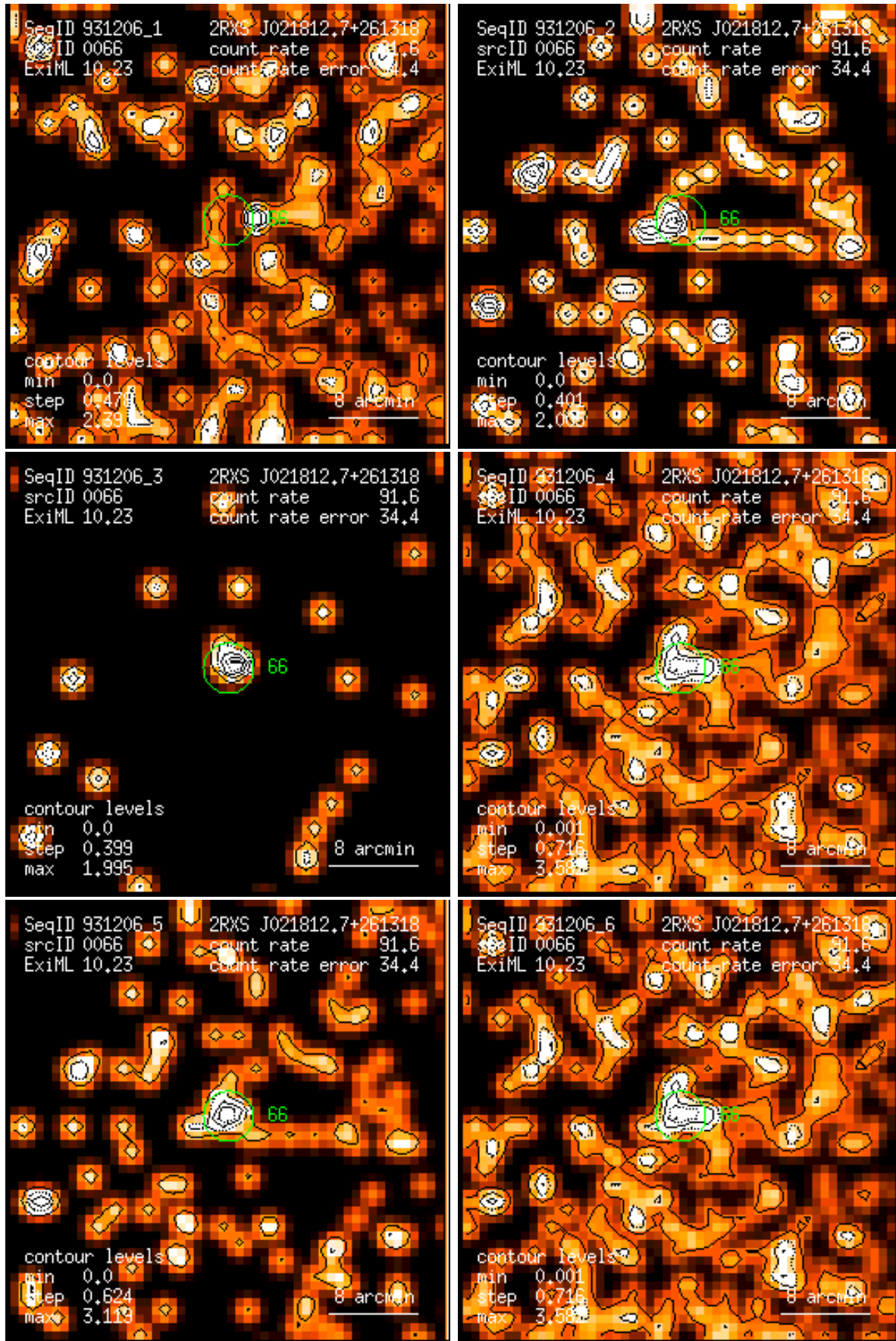
Figure 66: RASS 931206: detection 0066: band rate images, Gaussian filter: (1) PSPC channels 11 – 41, (2) 52 – 90, (3) 91 – 201, (4) 11 – 235, (5) 52 – 201, (6) 11 – 201. Broad band rates in counts/ks. Band rate contour levels in counts/ks/arcmin 2 .
