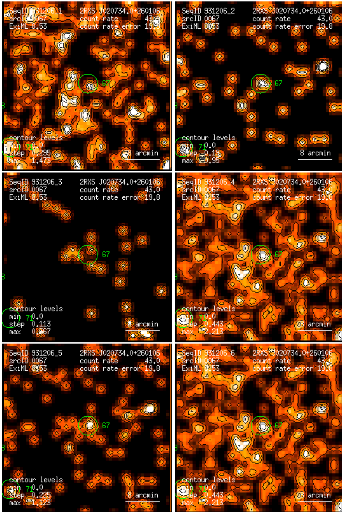
Figure 67: RASS 931206: detection 0067: band rate images, Gaussian filter: (1) PSPC channels 11 – 41, (2) 52 – 90, (3) 91 – 201, (4) 11 – 235, (5) 52 – 201, (6) 11 – 201. Broad band rates in counts/ks. Band rate contour levels in counts/ks/arcmin 2 .
