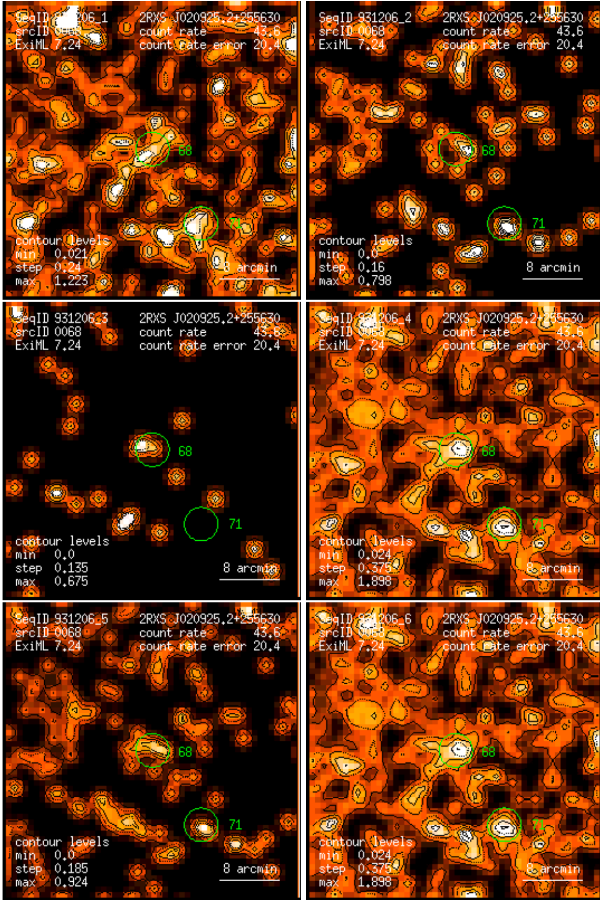
Figure 68: RASS 931206: detection 0068: band rate images, Gaussian filter: (1) PSPC channels 11 – 41, (2) 52 – 90, (3) 91 – 201, (4) 11 – 235, (5) 52 – 201, (6) 11 – 201. Broad band rates in counts/ks. Band rate contour levels in counts/ks/arcmin 2 .
