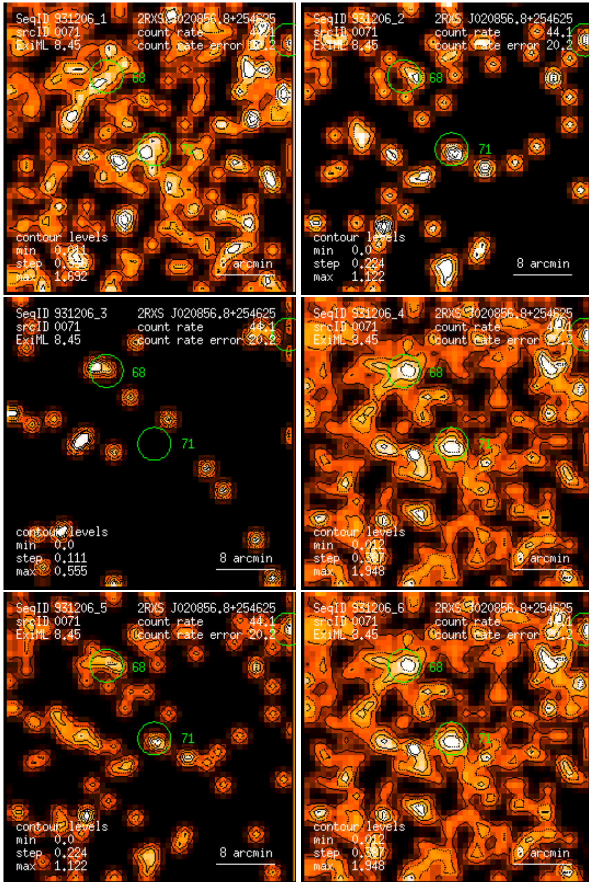
Figure 71: RASS 931206: detection 0071: band rate images, Gaussian filter: (1) PSPC channels 11 – 41, (2) 52 – 90, (3) 91 – 201, (4) 11 – 235, (5) 52 – 201, (6) 11 – 201. Broad band rates in counts/ks. Band rate contour levels in counts/ks/arcmin 2 .
