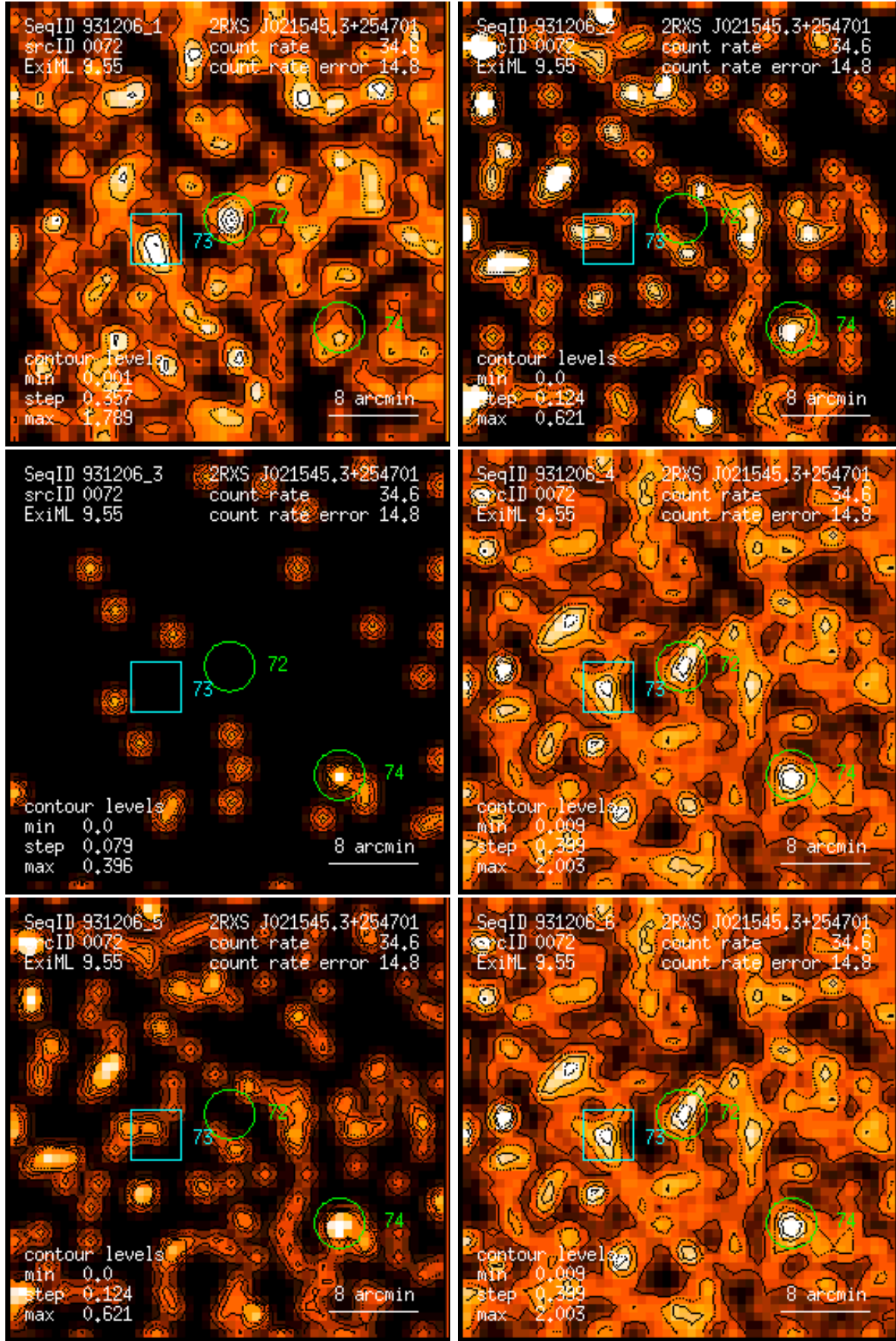
Figure 72: RASS 931206: detection 0072: band rate images, Gaussian filter: (1) PSPC channels 11 – 41, (2) 52 – 90, (3) 91 – 201, (4) 11 – 235, (5) 52 – 201, (6) 11 – 201. Broad band rates in counts/ks. Band rate contour levels in counts/ks/arcmin 2 .
