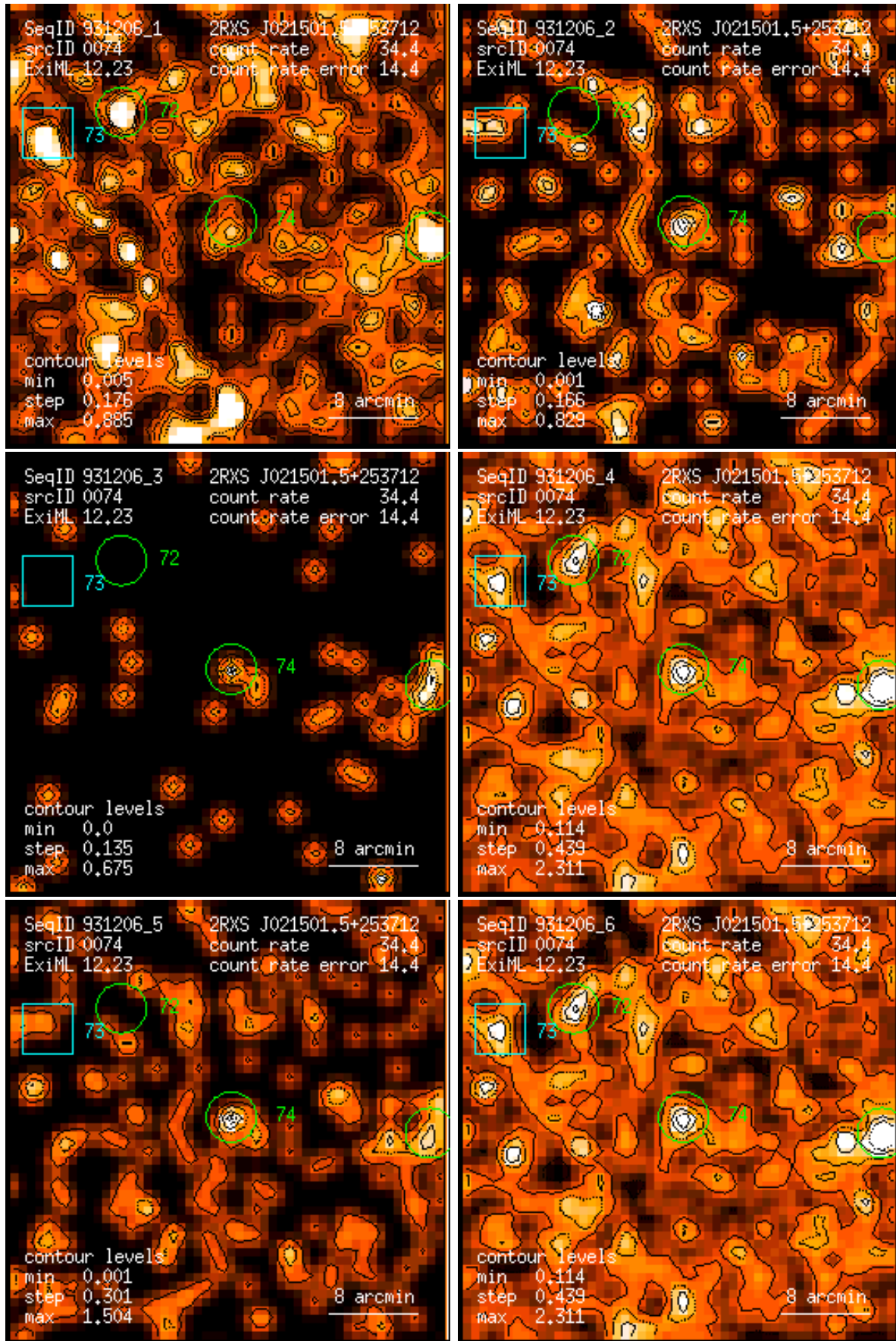
Figure 74: RASS 931206: detection 0074: band rate images, Gaussian filter: (1) PSPC channels 11 – 41, (2) 52 – 90, (3) 91 – 201, (4) 11 – 235, (5) 52 – 201, (6) 11 – 201. Broad band rates in counts/ks. Band rate contour levels in counts/ks/arcmin 2 .
