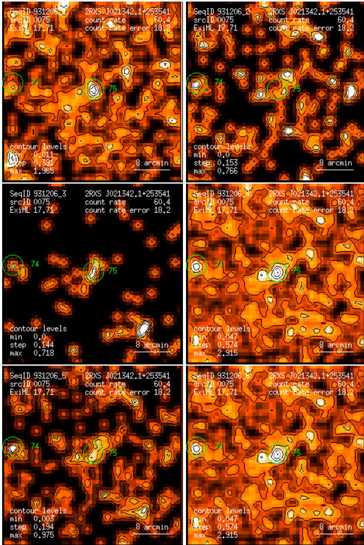
Figure 75: RASS 931206: detection 0075: band rate images, Gaussian filter: (1) PSPC channels 11 – 41, (2) 52 – 90, (3) 91 – 201, (4) 11 – 235, (5) 52 – 201, (6) 11 – 201. Broad band rates in counts/ks. Band rate contour levels in counts/ks/arcmin 2 .
