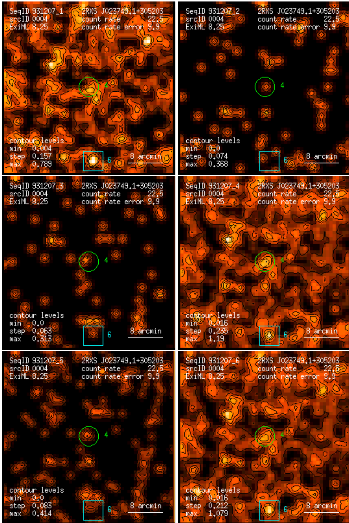
Figure 4: RASS 931207: detection 0004: band rate images, Gaussian filter: (1) PSPC channels 11 – 41, (2) 52 – 90, (3) 91 – 201, (4) 11 – 235, (5) 52 – 201, (6) 11 – 201. Broad band rates in counts/ks. Band rate contour levels in counts/ks/arcmin 2 .
