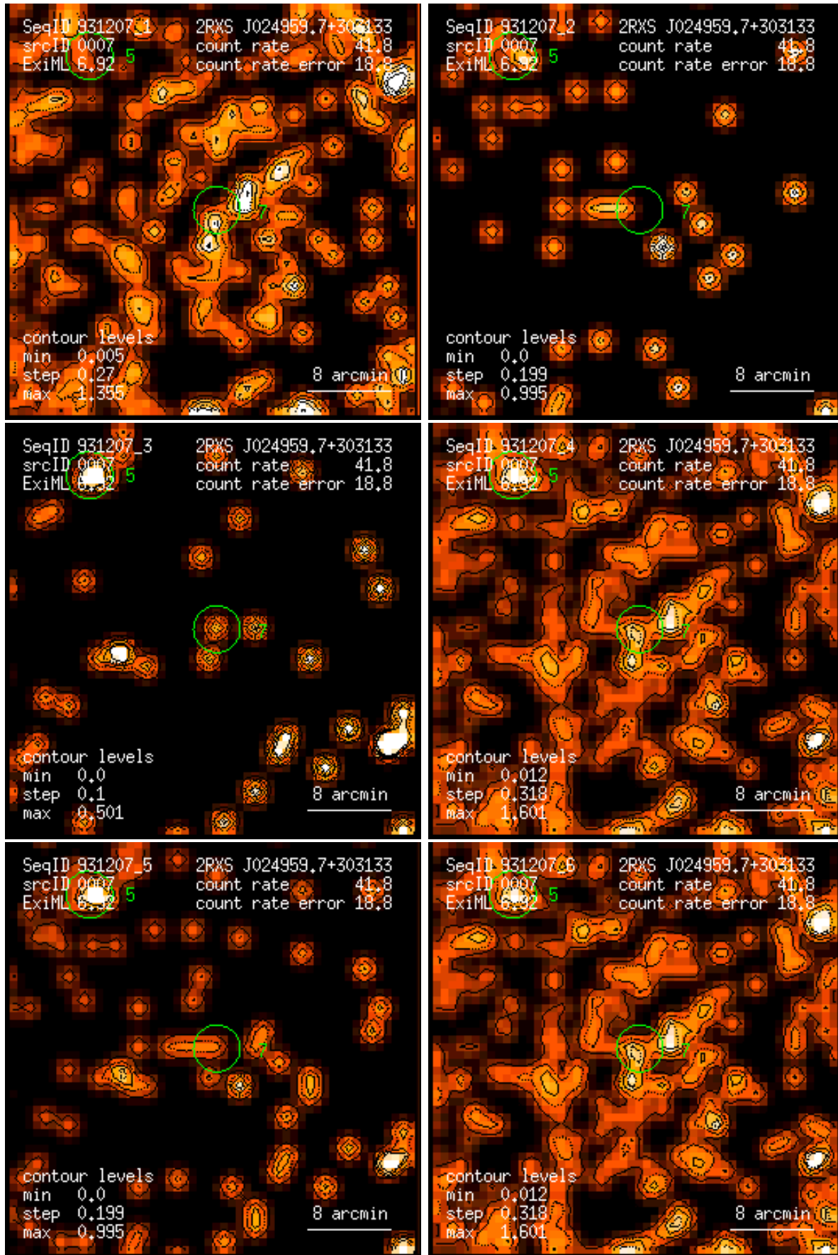
Figure 7: RASS 931207: detection 0007: band rate images, Gaussian filter: (1) PSPC channels 11 – 41, (2) 52 – 90, (3) 91 – 201, (4) 11 – 235, (5) 52 – 201, (6) 11 – 201. Broad band rates in counts/ks. Band rate contour levels in counts/ks/arcmin 2 .
