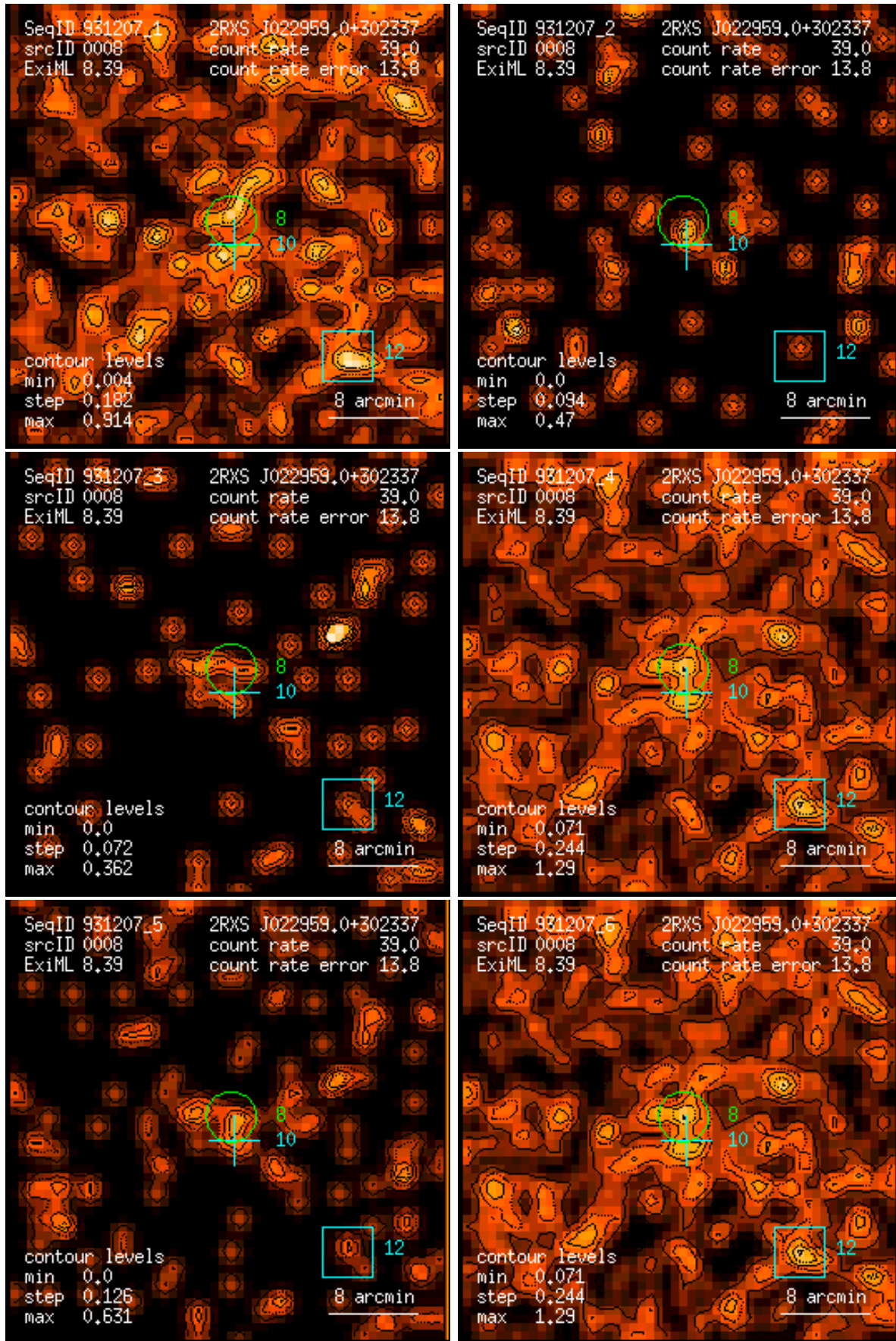
Figure 8: RASS 931207: detection 0008: band rate images, Gaussian filter: (1) PSPC channels 11 – 41, (2) 52 – 90, (3) 91 – 201, (4) 11 – 235, (5) 52 – 201, (6) 11 – 201. Broad band rates in counts/ks. Band rate contour levels in counts/ks/arcmin 2 .
