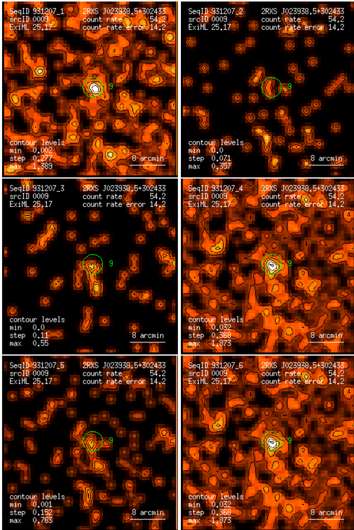
Figure 9: RASS 931207: detection 0009: band rate images, Gaussian filter: (1) PSPC channels 11 – 41, (2) 52 – 90, (3) 91 – 201, (4) 11 – 235, (5) 52 – 201, (6) 11 – 201. Broad band rates in counts/ks. Band rate contour levels in counts/ks/arcmin 2 .
