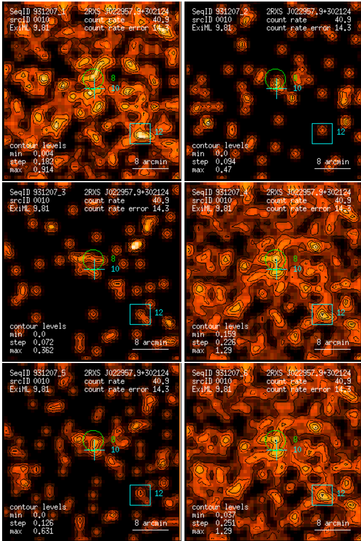
Figure 10: RASS 931207: detection 0010: band rate images, Gaussian filter: (1) PSPC channels 11 – 41, (2) 52 – 90, (3) 91 – 201, (4) 11 – 235, (5) 52 – 201, (6) 11 – 201. Broad band rates in counts/ks. Band rate contour levels in counts/ks/arcmin 2 .
