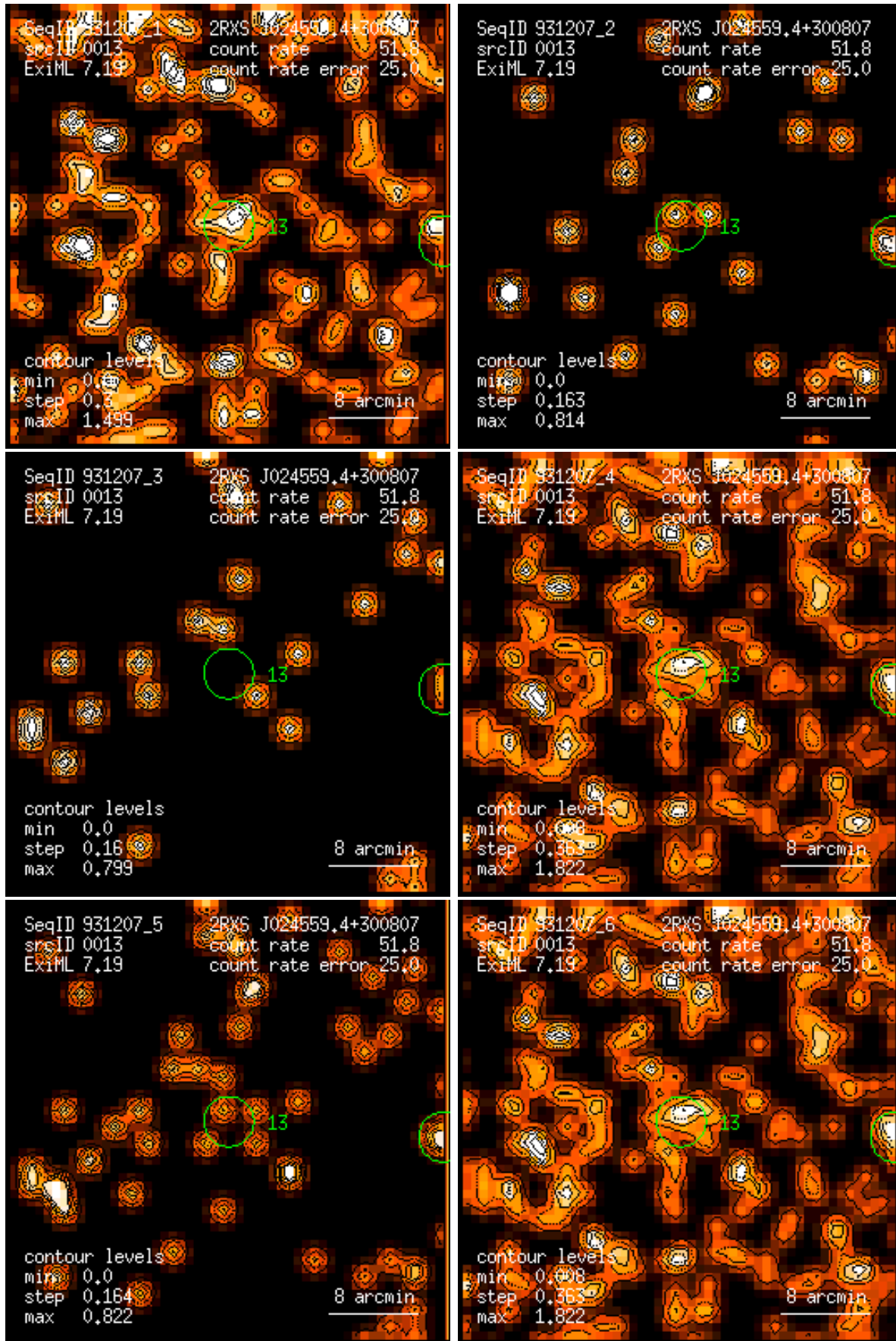
Figure 13: RASS 931207: detection 0013: band rate images, Gaussian filter: (1) PSPC channels 11 – 41, (2) 52 – 90, (3) 91 – 201, (4) 11 – 235, (5) 52 – 201, (6) 11 – 201. Broad band rates in counts/ks. Band rate contour levels in counts/ks/arcmin 2 .
