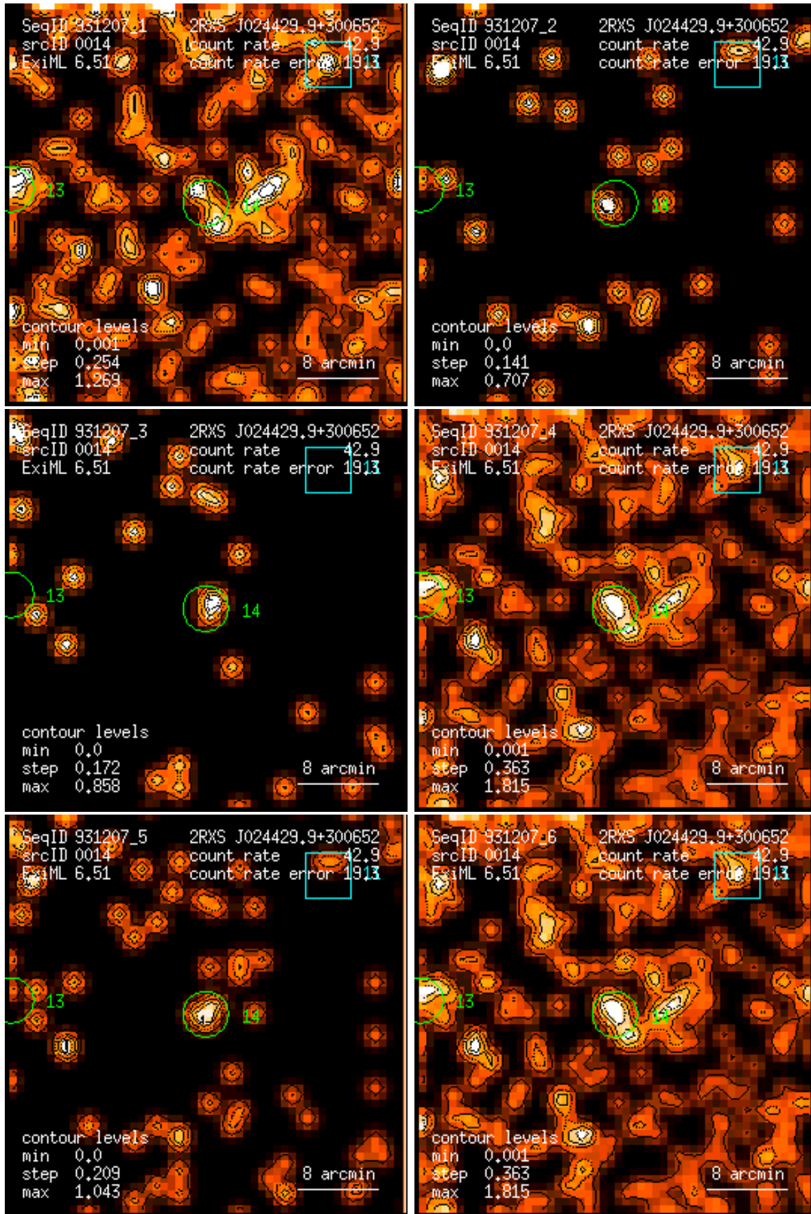
Figure 14: RASS 931207: detection 0014: band rate images, Gaussian filter: (1) PSPC channels 11 – 41, (2) 52 – 90, (3) 91 – 201, (4) 11 – 235, (5) 52 – 201, (6) 11 – 201. Broad band rates in counts/ks. Band rate contour levels in counts/ks/arcmin 2 .
