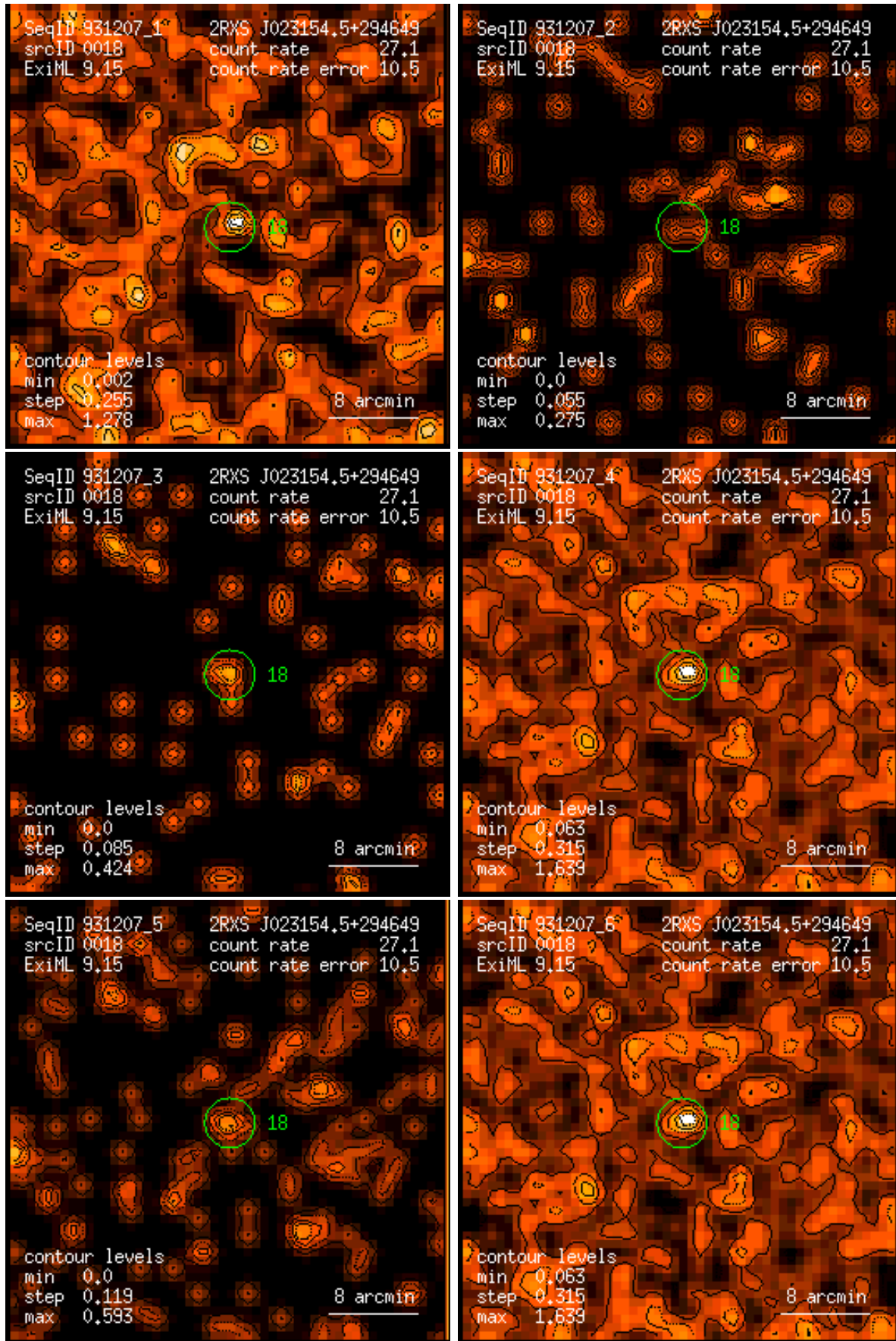
Figure 18: RASS 931207: detection 0018: band rate images, Gaussian filter: (1) PSPC channels 11 – 41, (2) 52 – 90, (3) 91 – 201, (4) 11 – 235, (5) 52 – 201, (6) 11 – 201. Broad band rates in counts/ks. Band rate contour levels in counts/ks/arcmin 2 .
