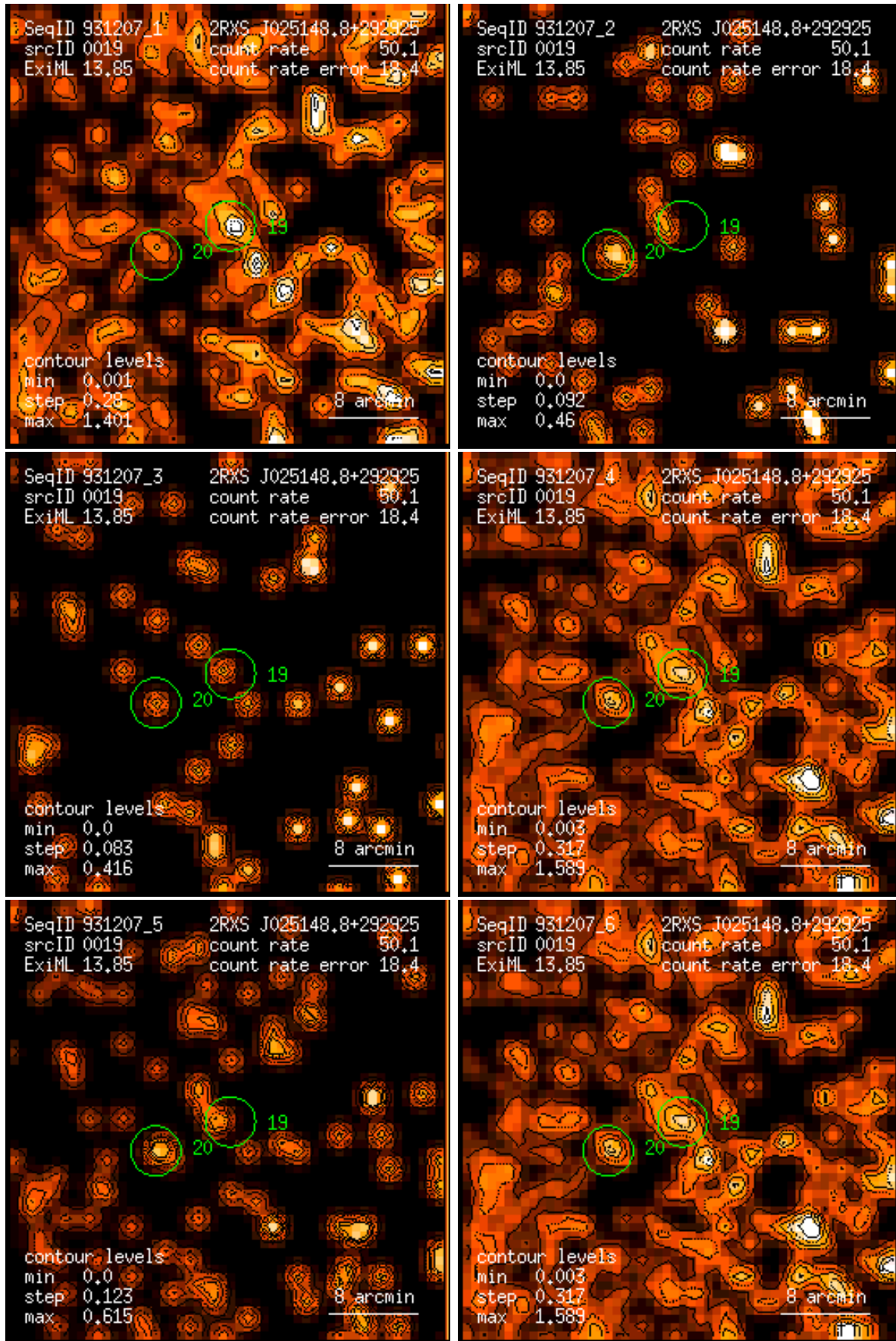
Figure 19: RASS 931207: detection 0019: band rate images, Gaussian filter: (1) PSPC channels 11 – 41, (2) 52 – 90, (3) 91 – 201, (4) 11 – 235, (5) 52 – 201, (6) 11 – 201. Broad band rates in counts/ks. Band rate contour levels in counts/ks/arcmin 2 .
