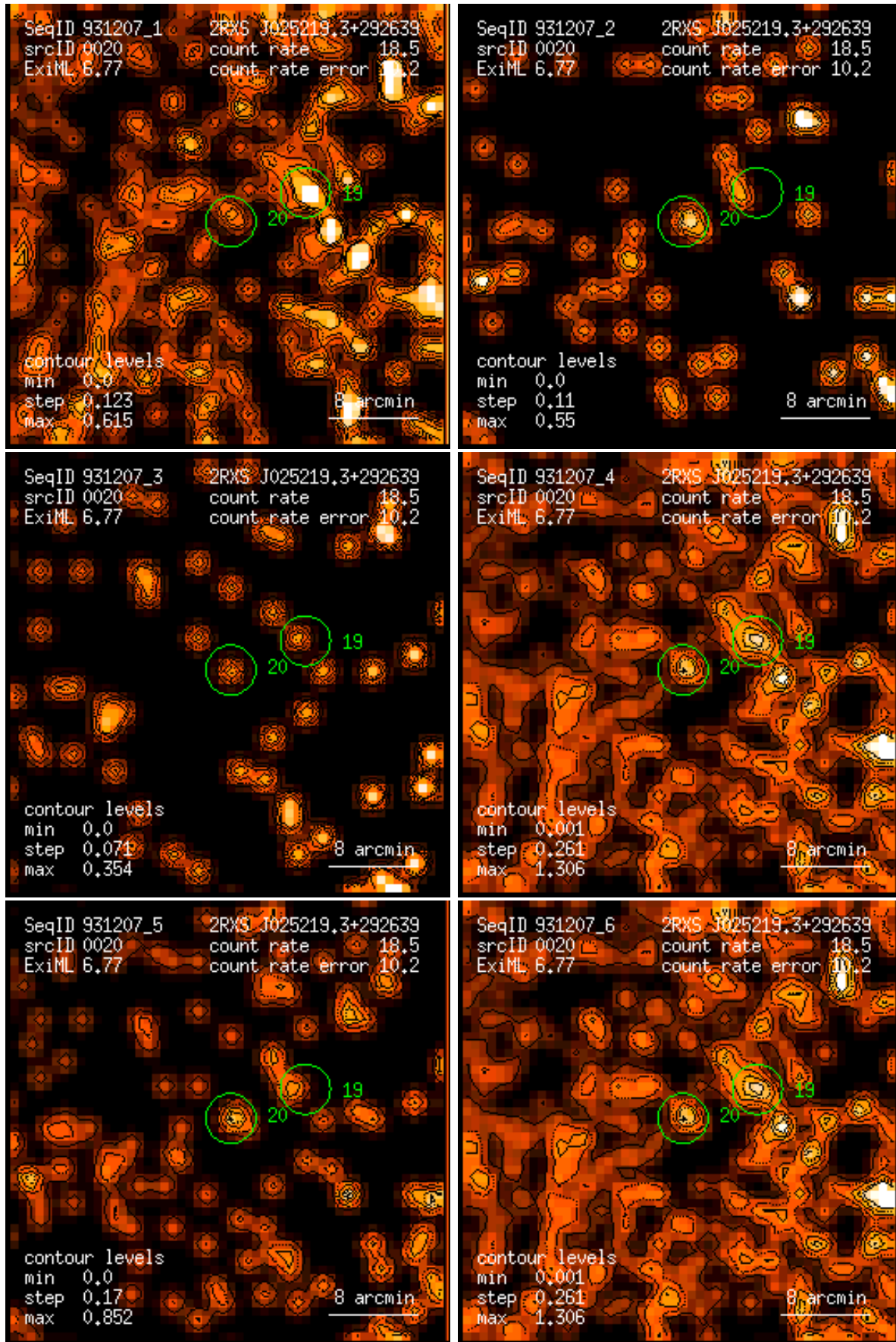
Figure 20: RASS 931207: detection 0020: band rate images, Gaussian filter: (1) PSPC channels 11 – 41, (2) 52 – 90, (3) 91 – 201, (4) 11 – 235, (5) 52 – 201, (6) 11 – 201. Broad band rates in counts/ks. Band rate contour levels in counts/ks/arcmin 2 .
