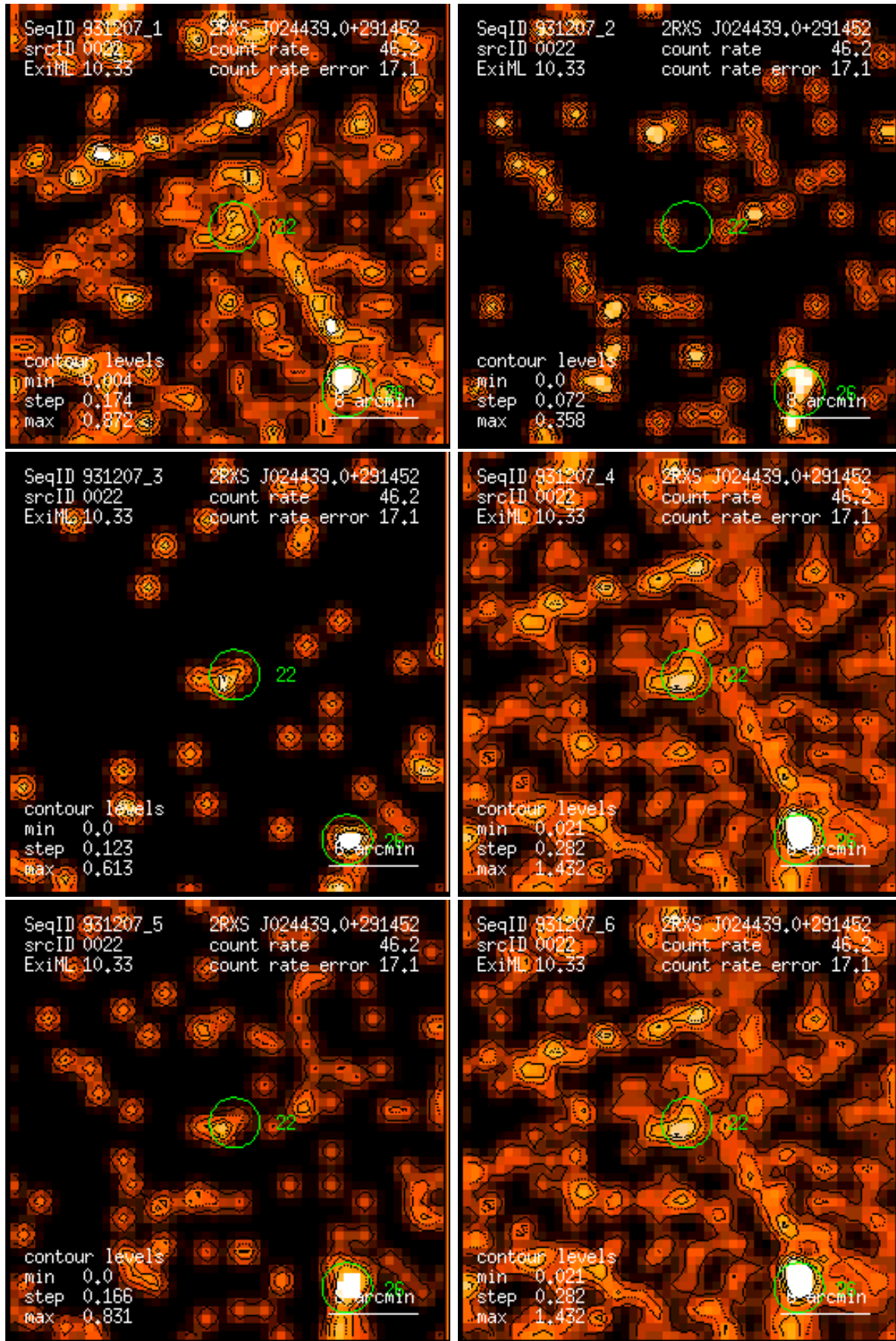
Figure 22: RASS 931207: detection 0022: band rate images, Gaussian filter: (1) PSPC channels 11 – 41, (2) 52 – 90, (3) 91 – 201, (4) 11 – 235, (5) 52 – 201, (6) 11 – 201. Broad band rates in counts/ks. Band rate contour levels in counts/ks/arcmin 2 .
