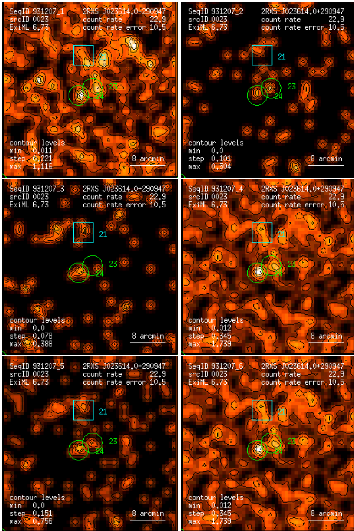
Figure 23: RASS 931207: detection 0023: band rate images, Gaussian filter: (1) PSPC channels 11 – 41, (2) 52 – 90, (3) 91 – 201, (4) 11 – 235, (5) 52 – 201, (6) 11 – 201. Broad band rates in counts/ks. Band rate contour levels in counts/ks/arcmin 2 .
