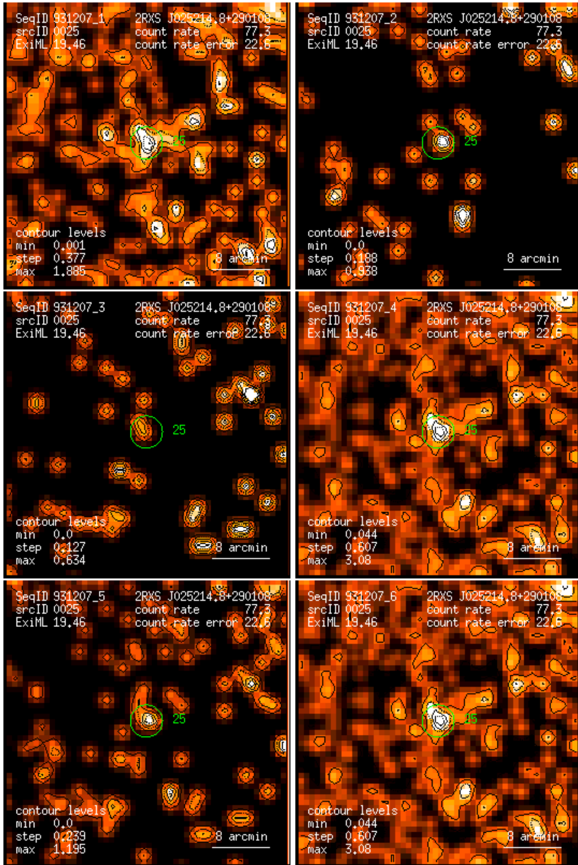
Figure 25: RASS 931207: detection 0025: band rate images, Gaussian filter: (1) PSPC channels 11 – 41, (2) 52 – 90, (3) 91 – 201, (4) 11 – 235, (5) 52 – 201, (6) 11 – 201. Broad band rates in counts/ks. Band rate contour levels in counts/ks/arcmin 2 .
