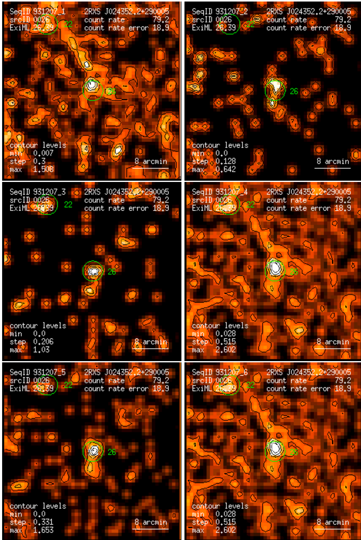
Figure 26: RASS 931207: detection 0026: band rate images, Gaussian filter: (1) PSPC channels 11 – 41, (2) 52 – 90, (3) 91 – 201, (4) 11 – 235, (5) 52 – 201, (6) 11 – 201. Broad band rates in counts/ks. Band rate contour levels in counts/ks/arcmin 2 .
