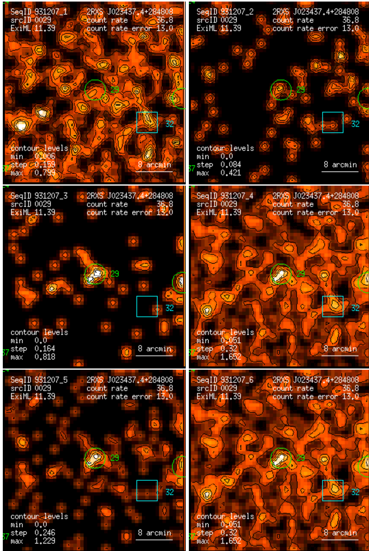
Figure 29: RASS 931207: detection 0029: band rate images, Gaussian filter: (1) PSPC channels 11 – 41, (2) 52 – 90, (3) 91 – 201, (4) 11 – 235, (5) 52 – 201, (6) 11 – 201. Broad band rates in counts/ks. Band rate contour levels in counts/ks/arcmin 2 .
