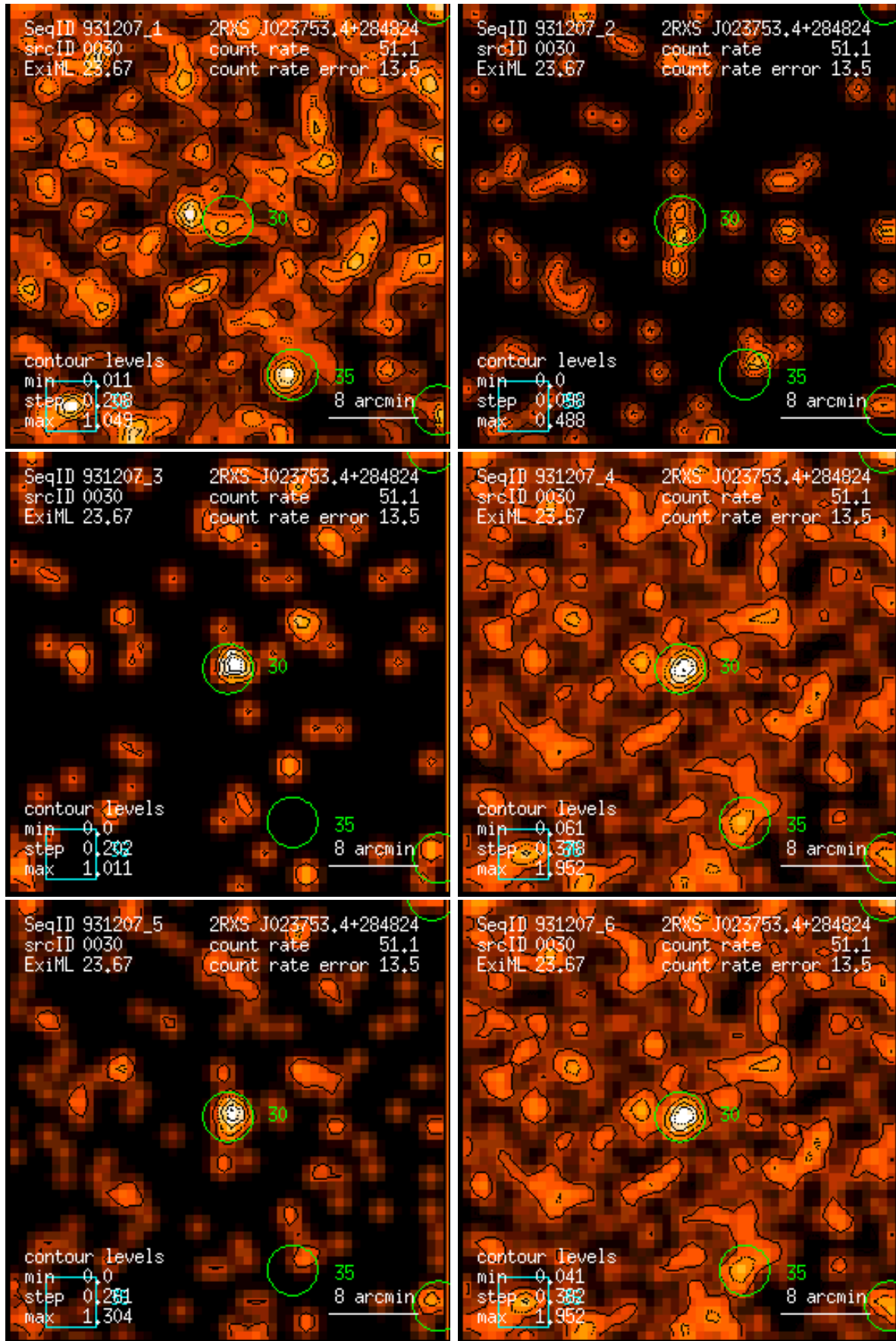
Figure 30: RASS 931207: detection 0030: band rate images, Gaussian filter: (1) PSPC channels 11 – 41, (2) 52 – 90, (3) 91 – 201, (4) 11 – 235, (5) 52 – 201, (6) 11 – 201. Broad band rates in counts/ks. Band rate contour levels in counts/ks/arcmin 2 .
