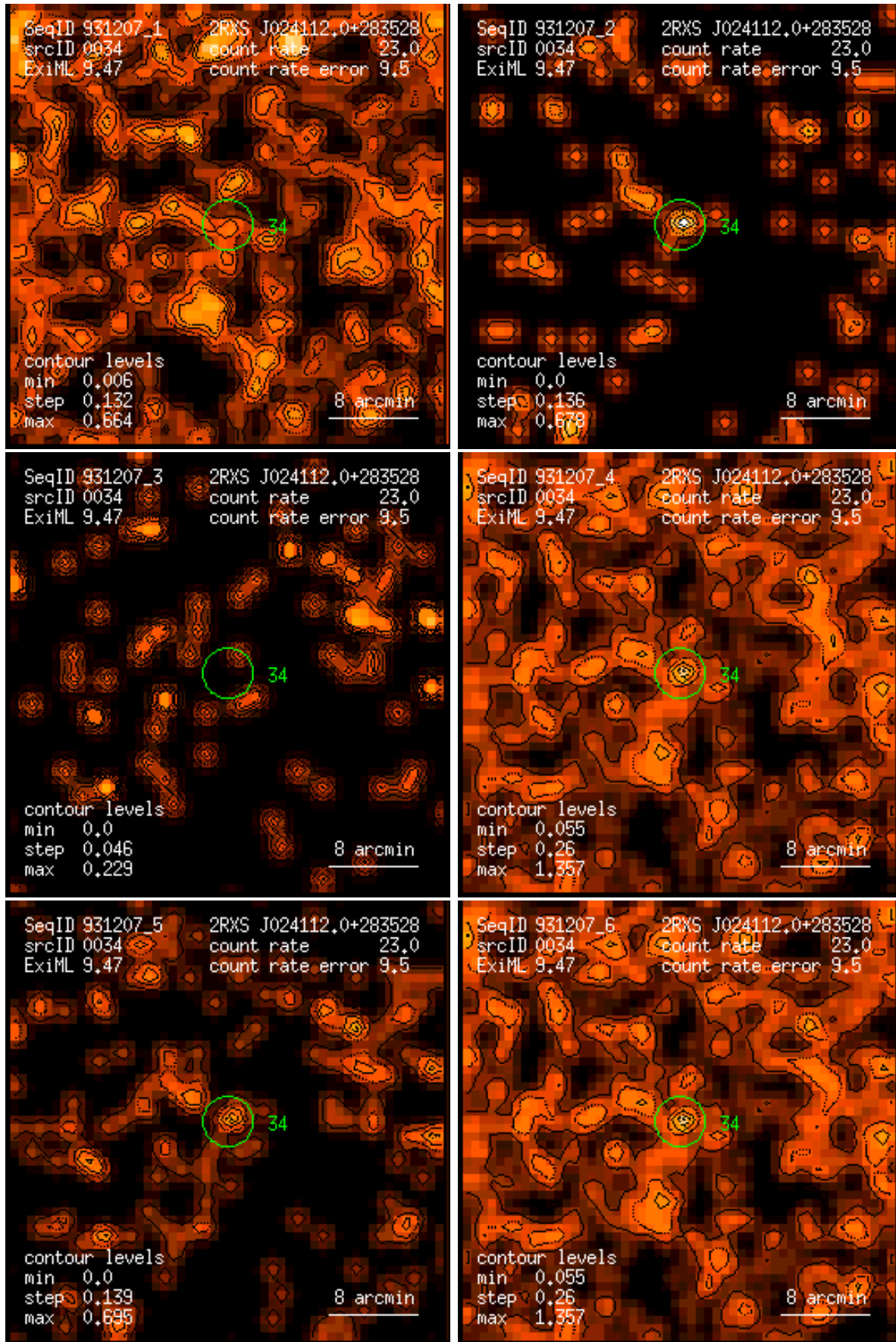
Figure 34: RASS 931207: detection 0034: band rate images, Gaussian filter: (1) PSPC channels 11 – 41, (2) 52 – 90, (3) 91 – 201, (4) 11 – 235, (5) 52 – 201, (6) 11 – 201. Broad band rates in counts/ks. Band rate contour levels in counts/ks/arcmin 2 .
